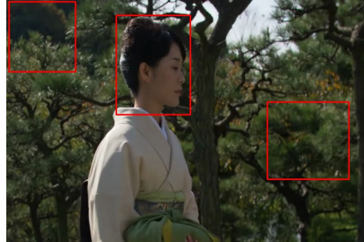
ActDiff-VC (0.0247 / 0.226 / 28.55 )
