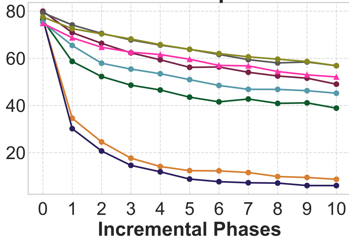
Cifar-100 10 phases
