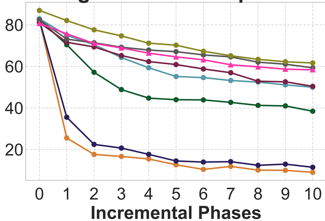
ImagNet-Subset 10 phases
