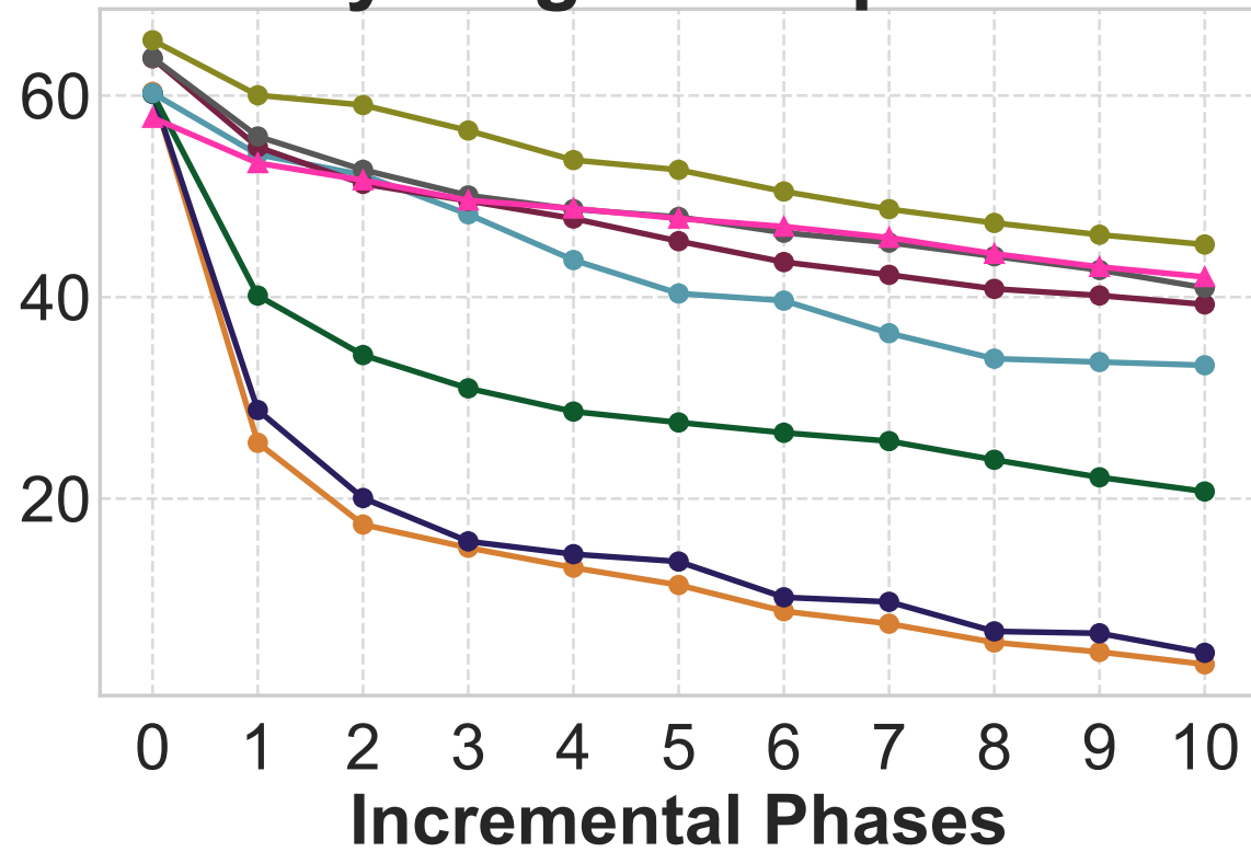
TinyImagNet 10 phases
