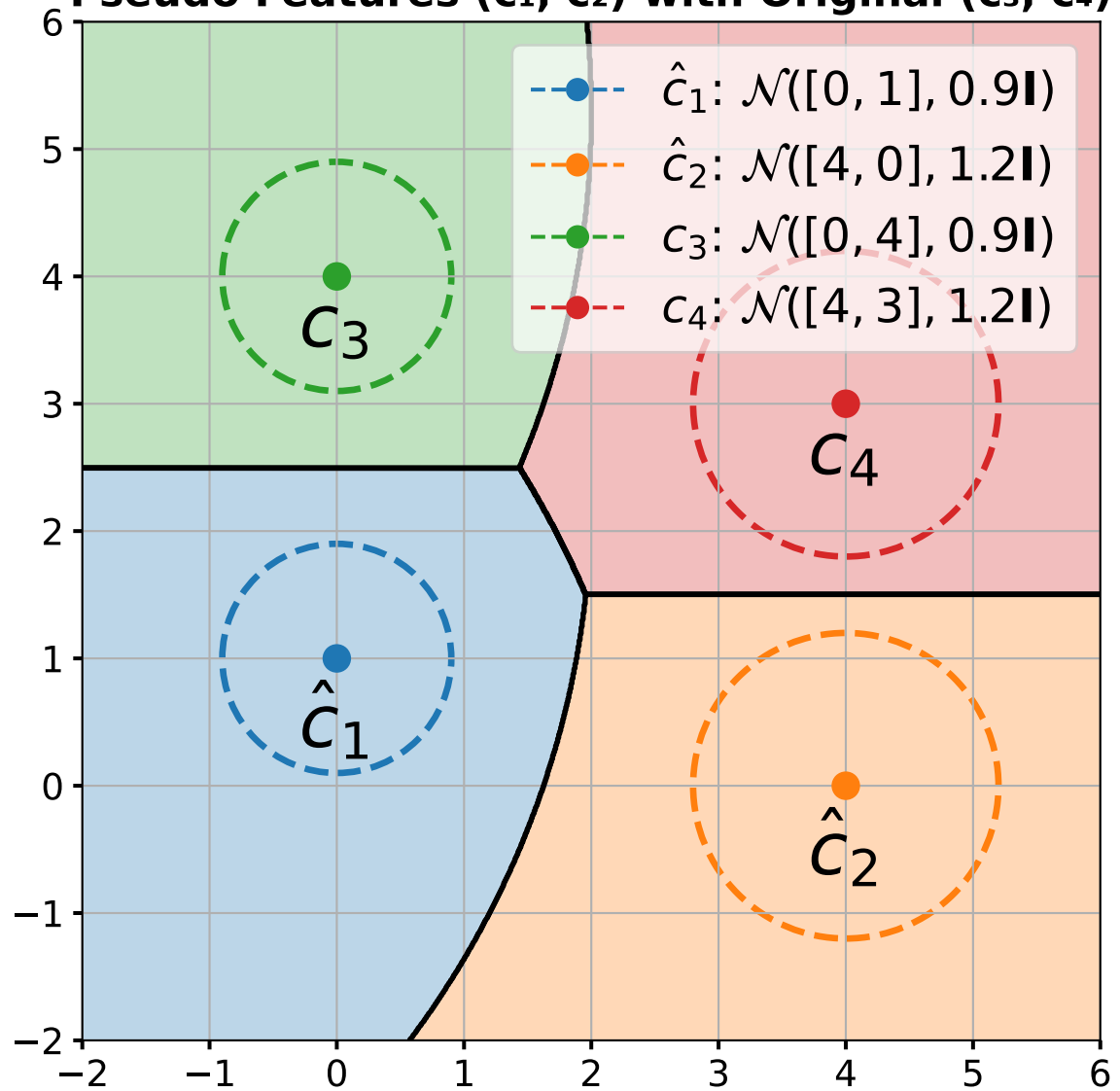
Pseudo Features ( \hat{c}_1, \hat{c}_2 ) with Original ( c_3, c_4 )
