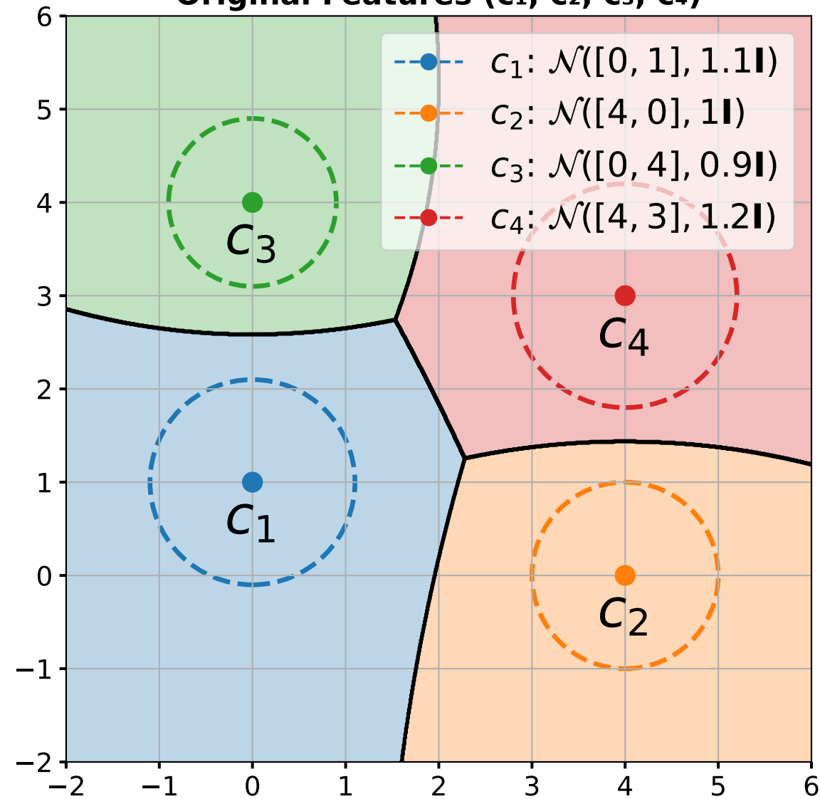
Original Features ( c_1, c_2, c_3, c_4 )
