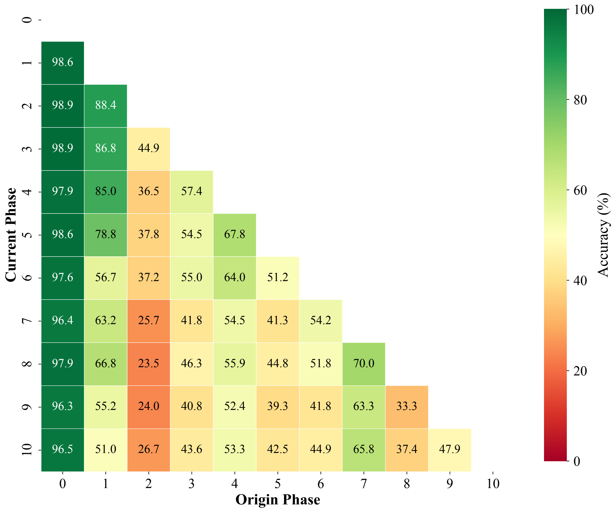
Pseudo-feature Accuracy
