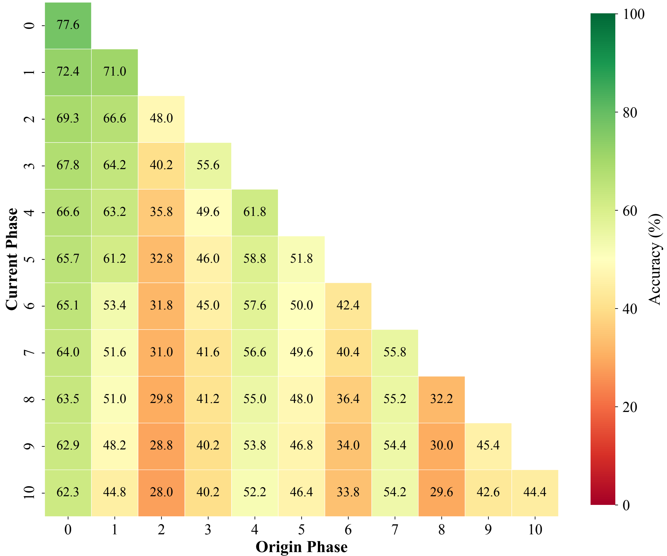
Test Accuracy
