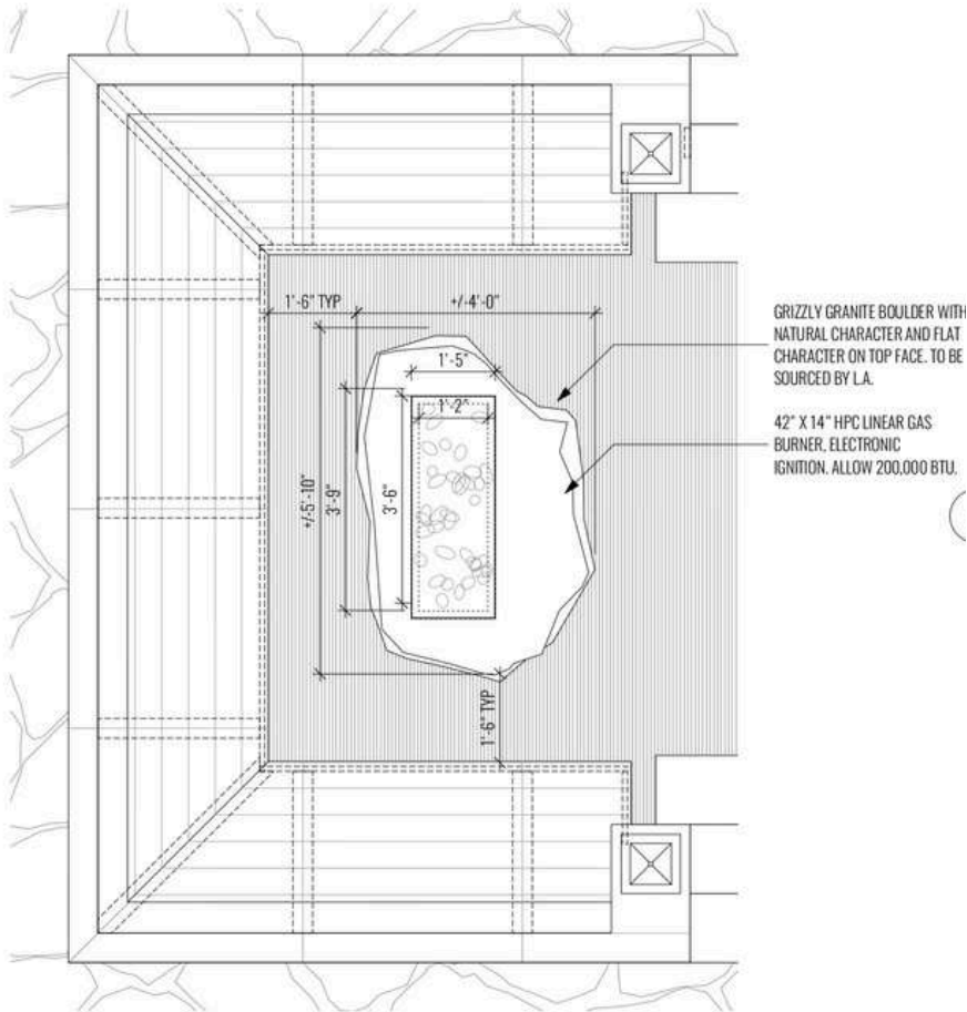
9 PLAN VIEW, FIREPIT Scale: 1/2" = 1'-0"
