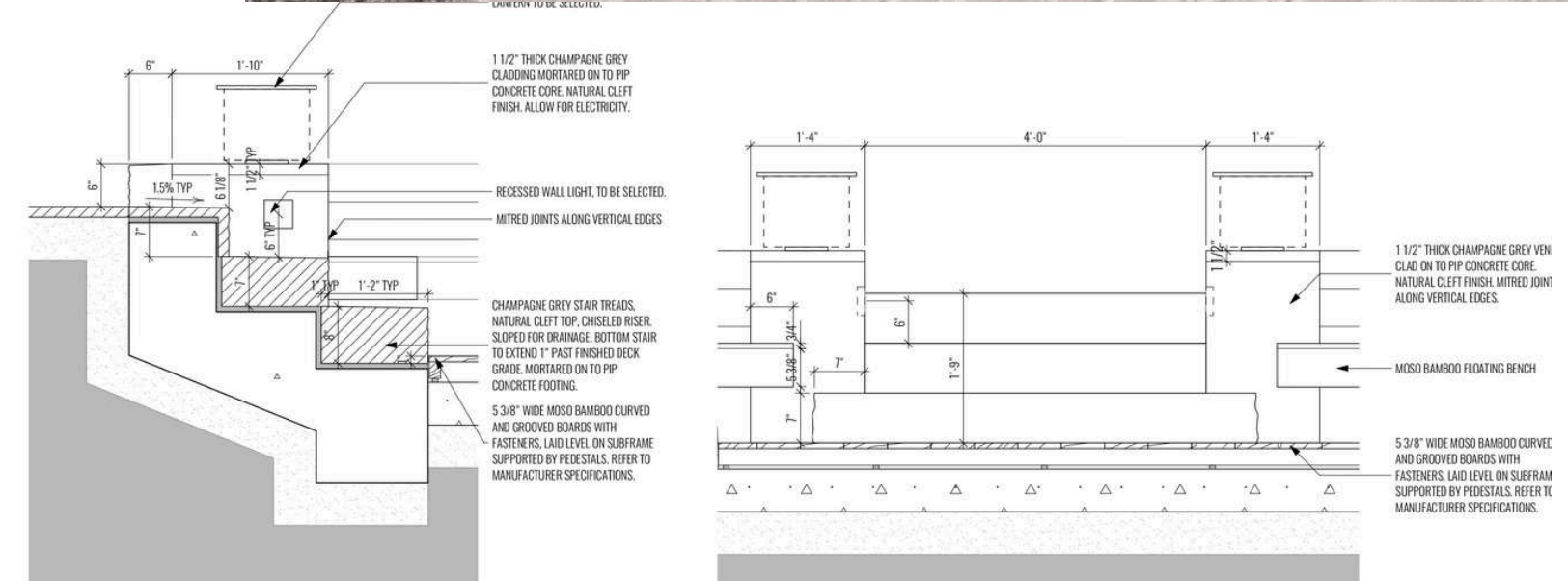
7 DETAIL E-E, STONE STAIRS Scale: 1" = 1'-0"
