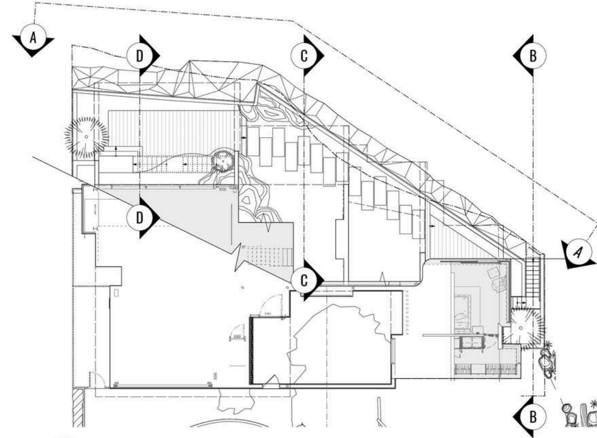
KEY PLAN Scale: 3/32" = 1' -0"
