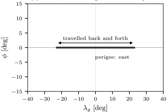
(c) i = 0 , e = 0.2 : segment on the equator
