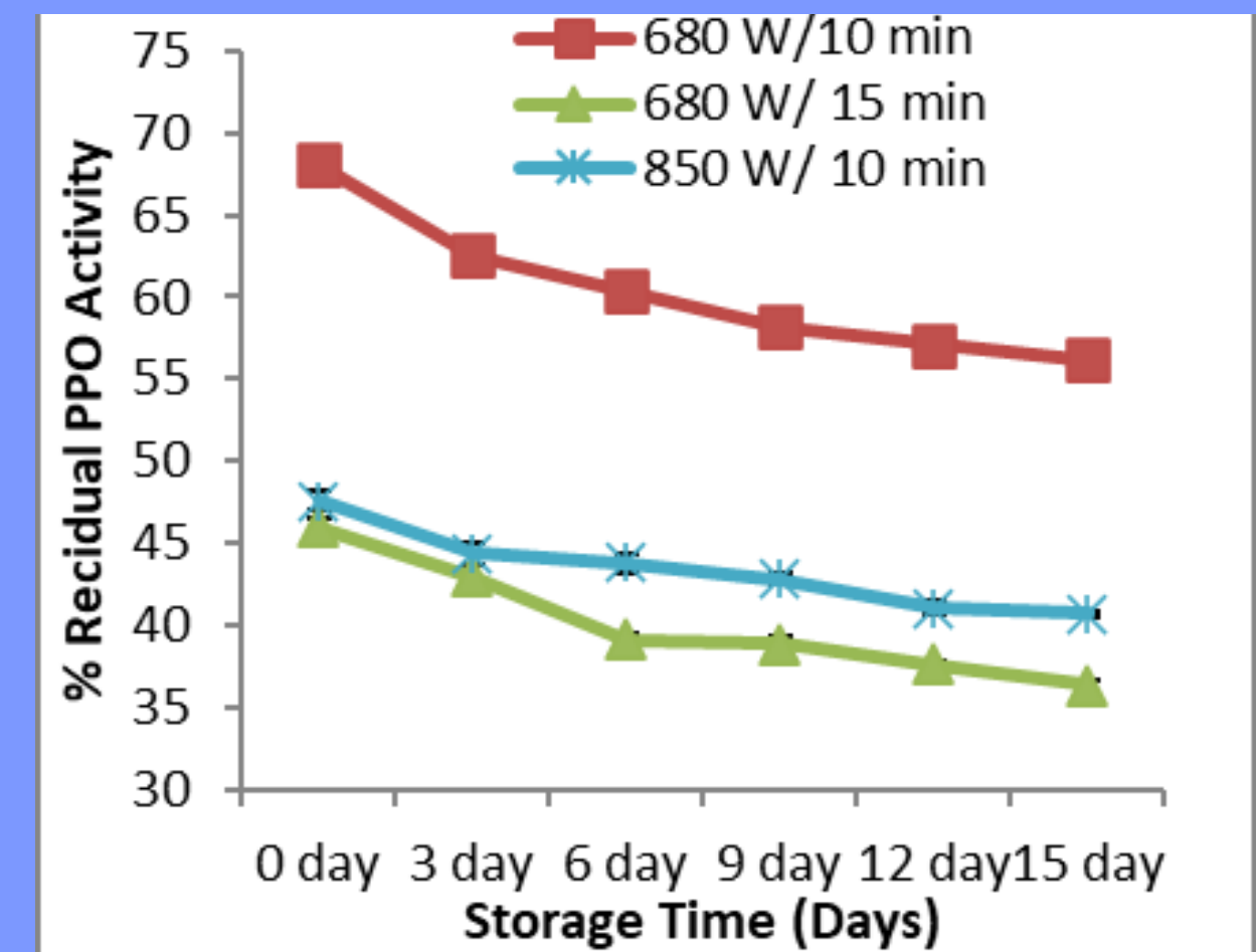
Fig ; Effect of refrigerated storage of the microwave heated sugarcane juice on polyphenol activity
