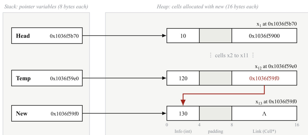
Figure 3: Memory during the final step of the insertion, using addresses from the program run. The pointers are on the stack; the cells are on the heap. The Link of x12 now holds 0x1036f59f0 , the address of New .
