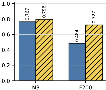
(b) Recall
