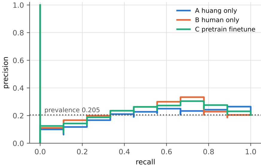
Precision-recall on the temporal test set (n=44, 9 positive)
