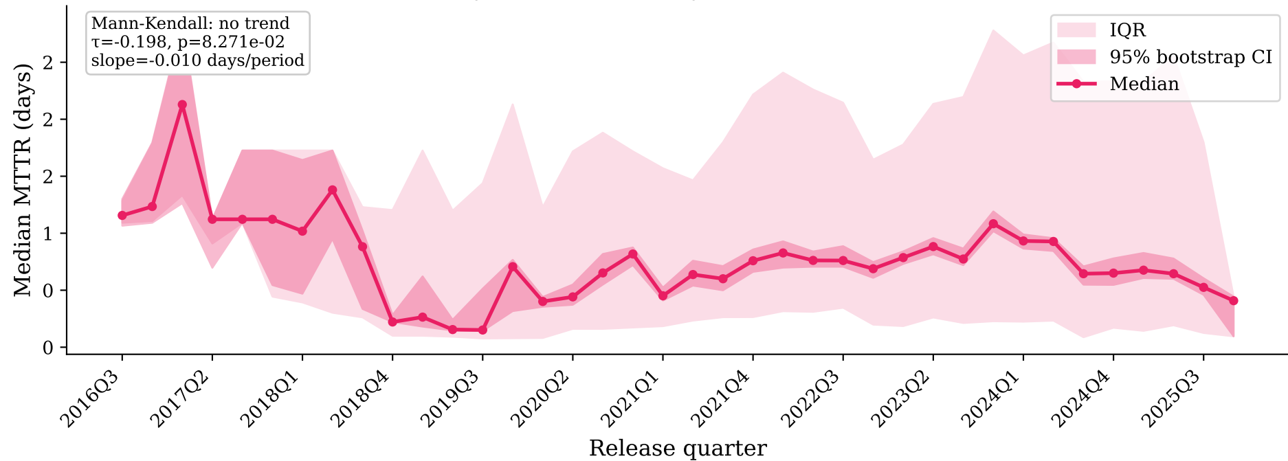
PyPI MTTR trend by release quarter
