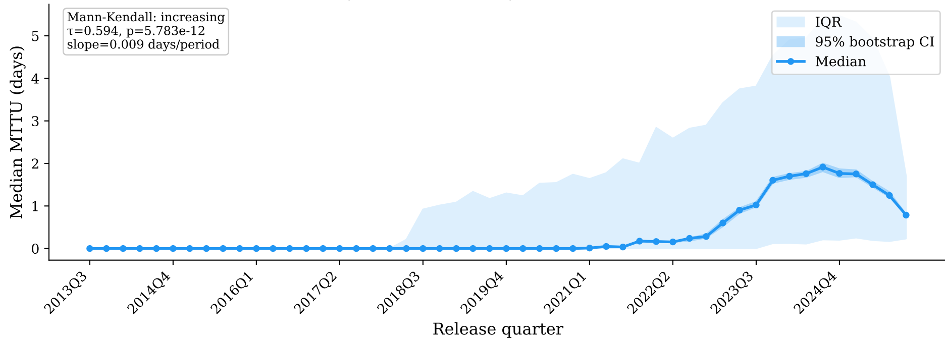
PyPI MTTU trend by release quarter
