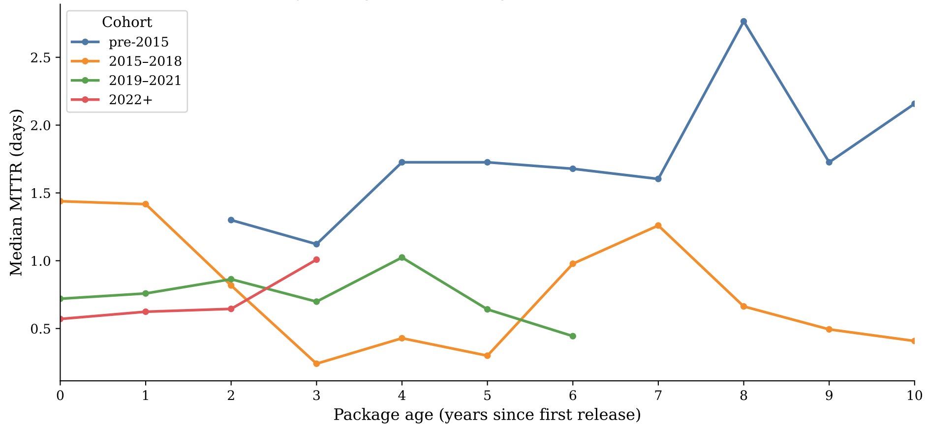
MTTR by package cohort and age (non-zero MTTR releases)
