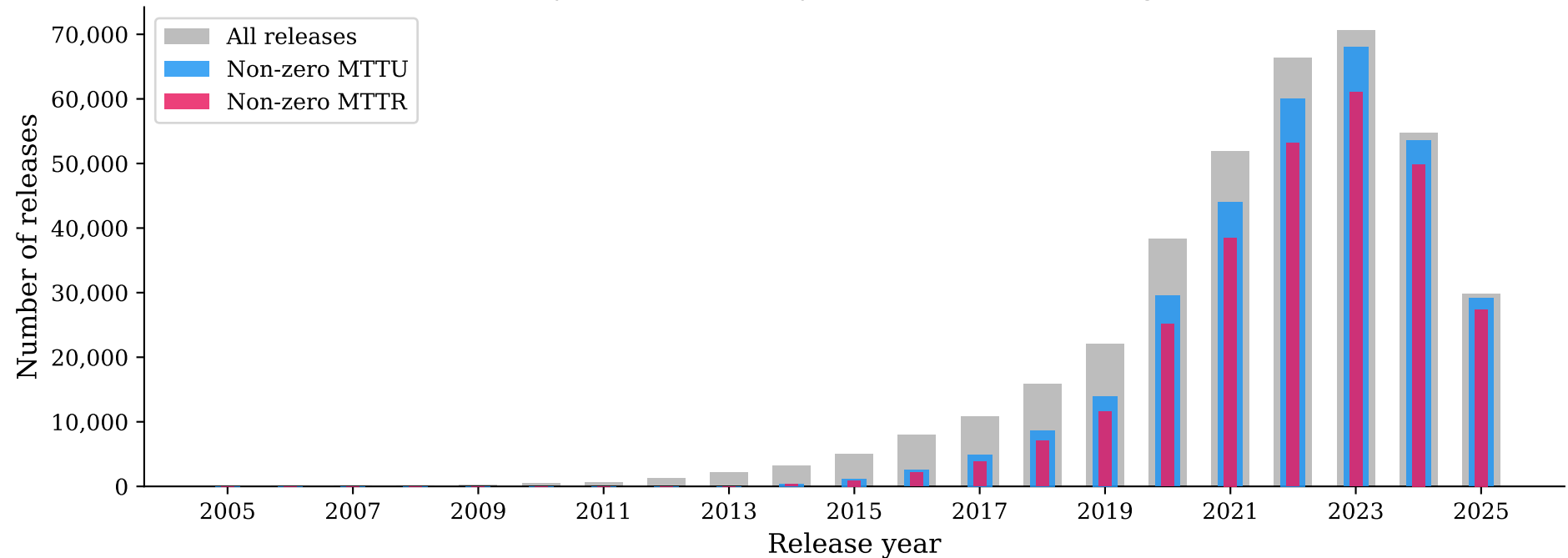
PyPI releases per year and metric coverage
