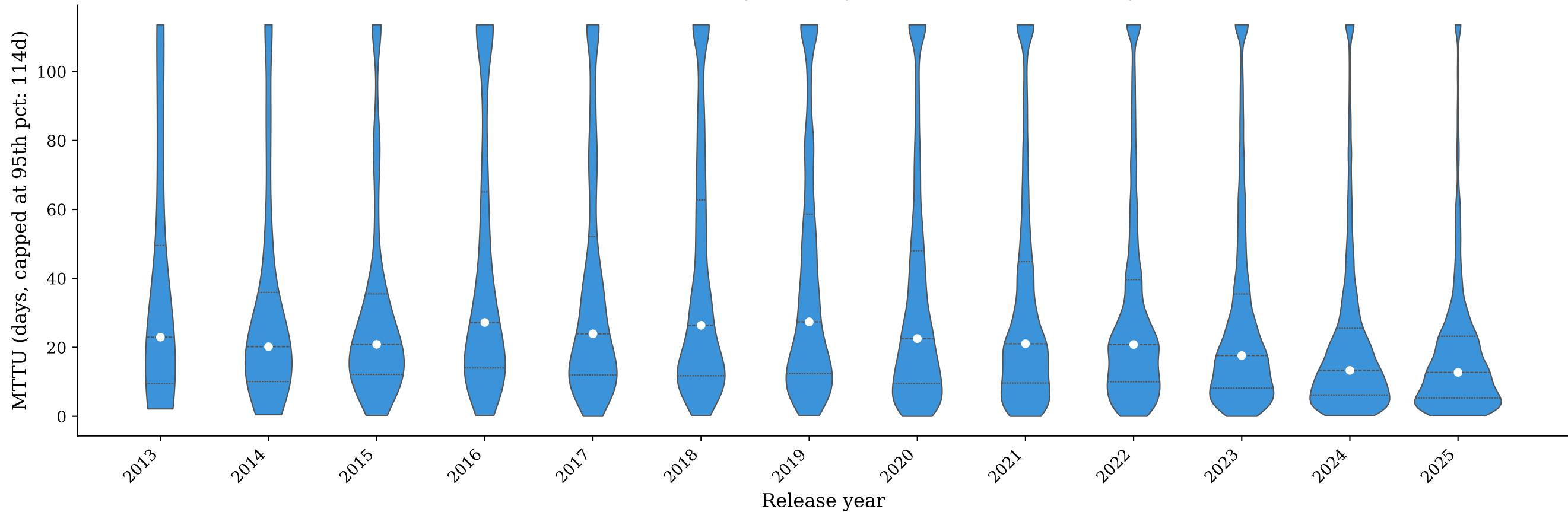
Distribution of MTTU by release year (non-zero releases only)
