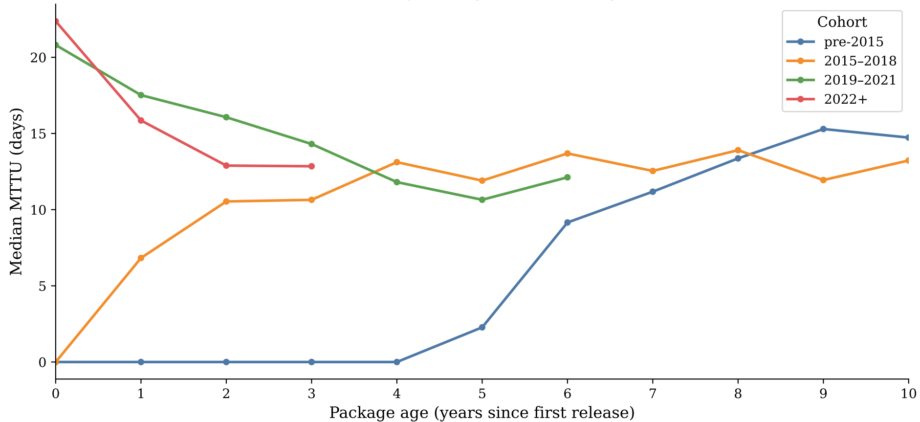
MTTU by package cohort and age
