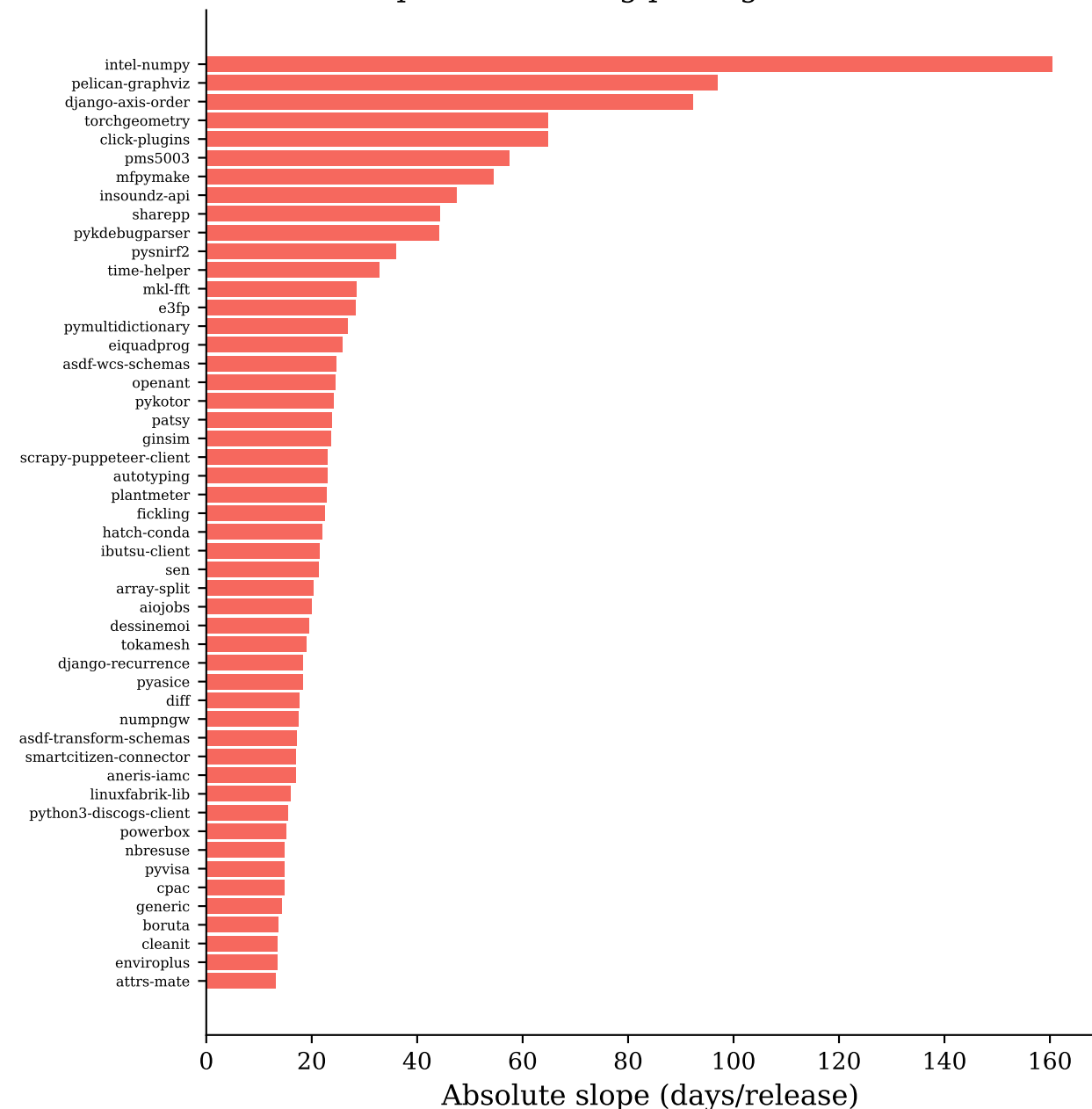
Top 50 Worsening packages — MTTR
