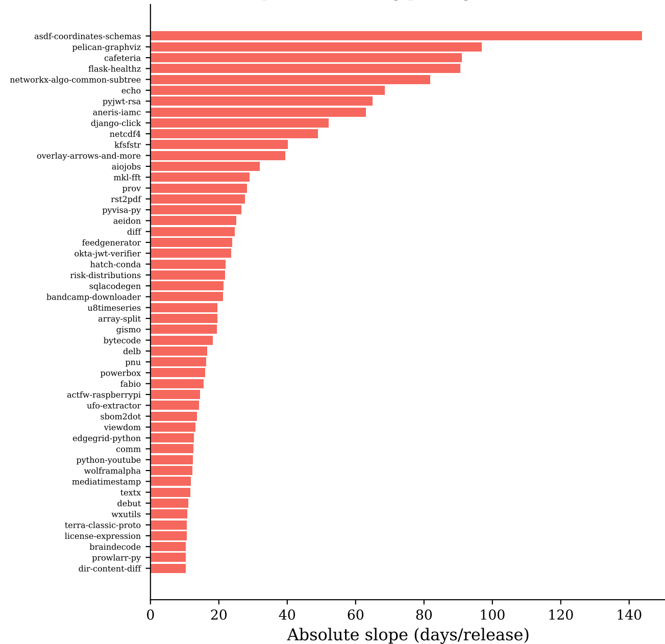
Top 50 Worsening packages — MTTR
