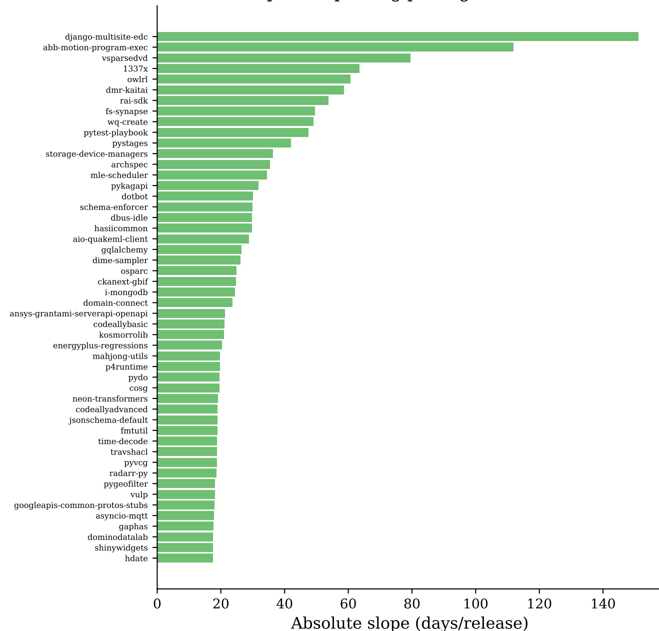
Top 50 Improving packages — MTTR
