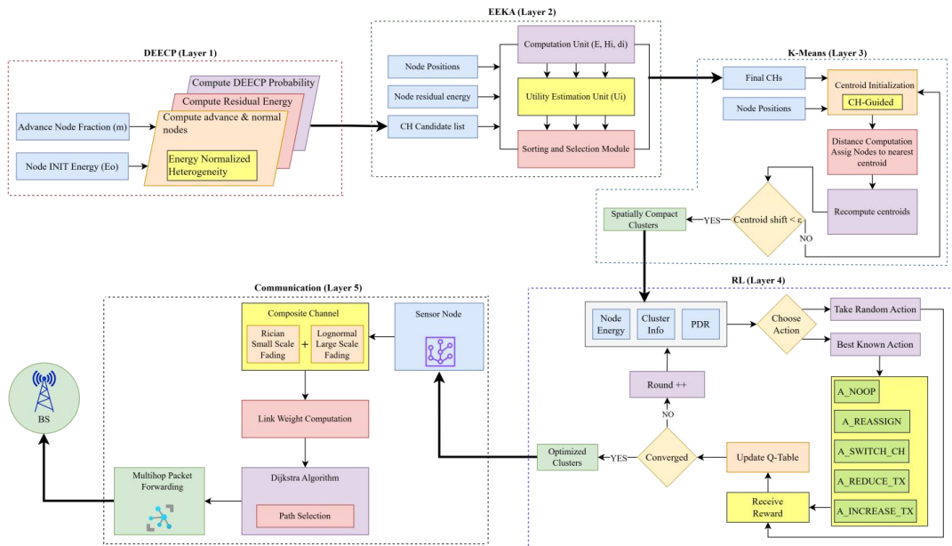
Figure 3.1 End-to-End Layer Integration
