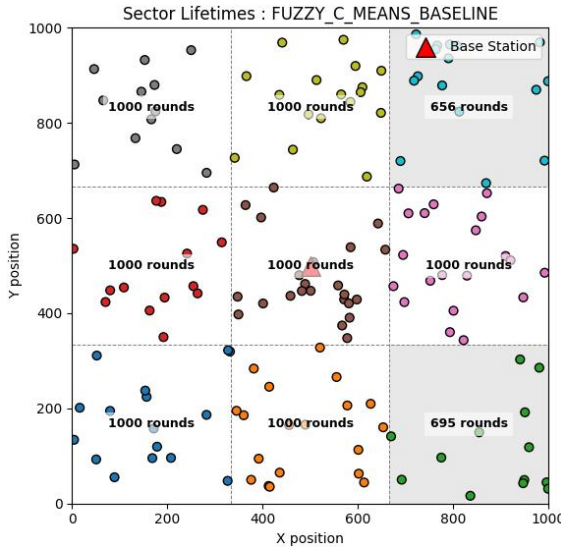
Fig 4.3 Sector-wise survival in FCM
