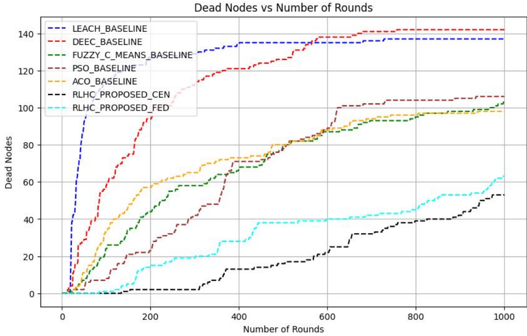
Figure 4.2.1 Network lifetime in terms of node death
