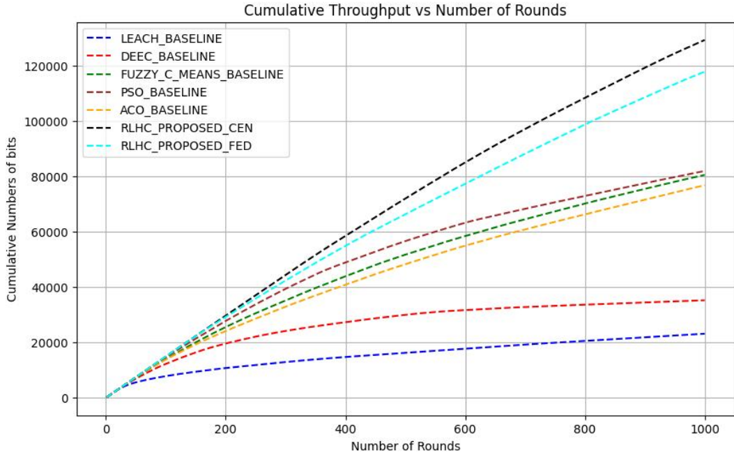
Figure 4.4 Cumulative Throughput
