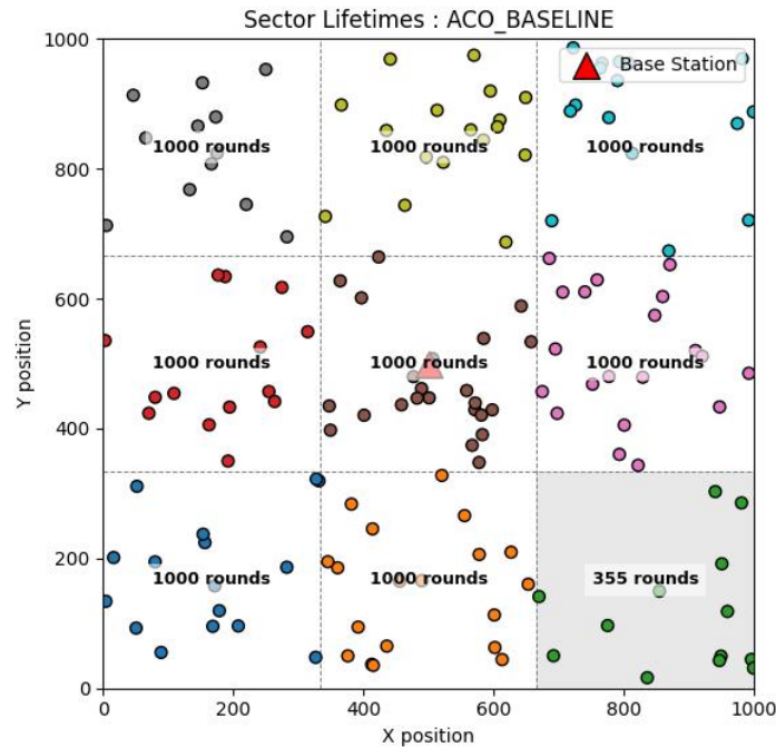
Fig 4.5 Sector-wise survival in ACO
