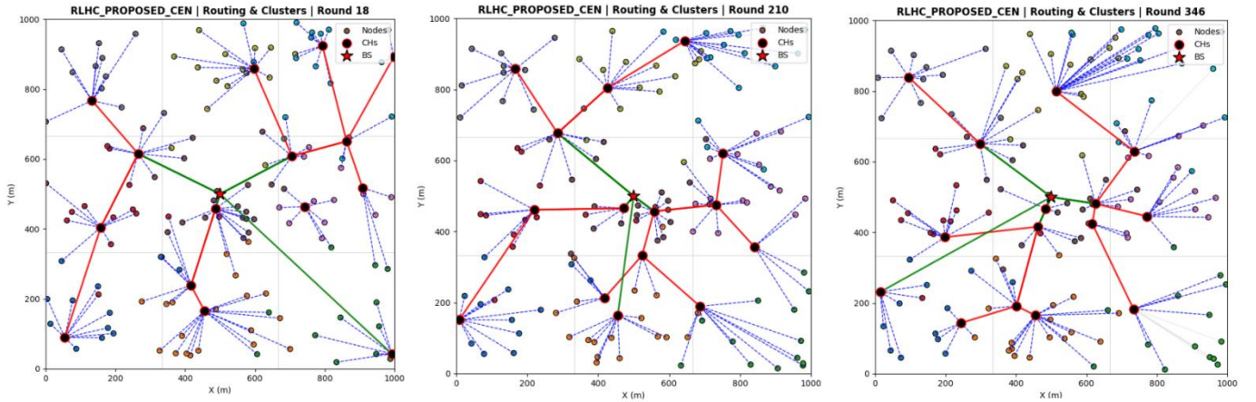
Figure 3.7 Simulation of the RLHC framework illustrating mobile sensor nodes and multi-hop communication
