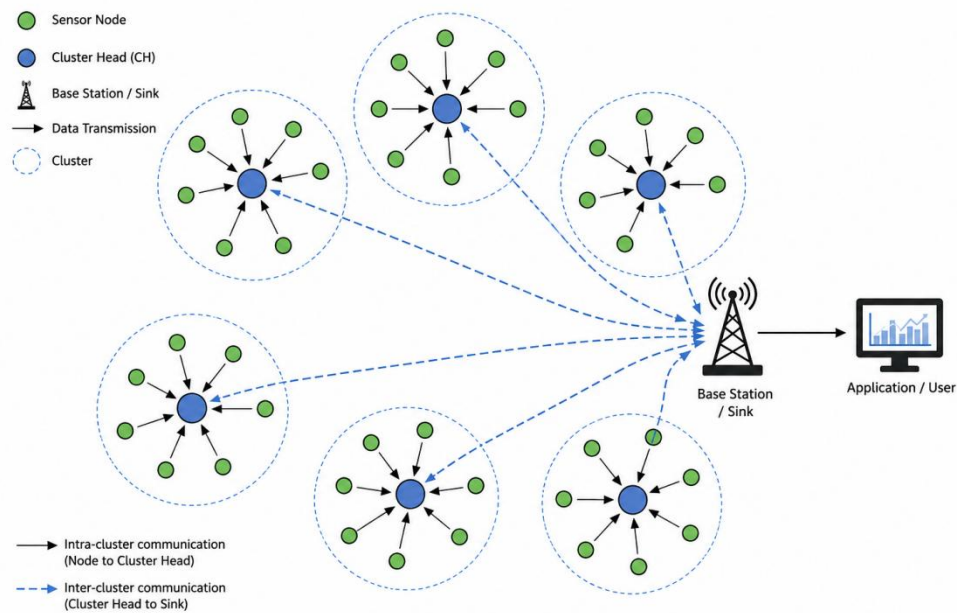
Figure 2.1.1 Representation of the LEACH WSNs for data gathering [5].
