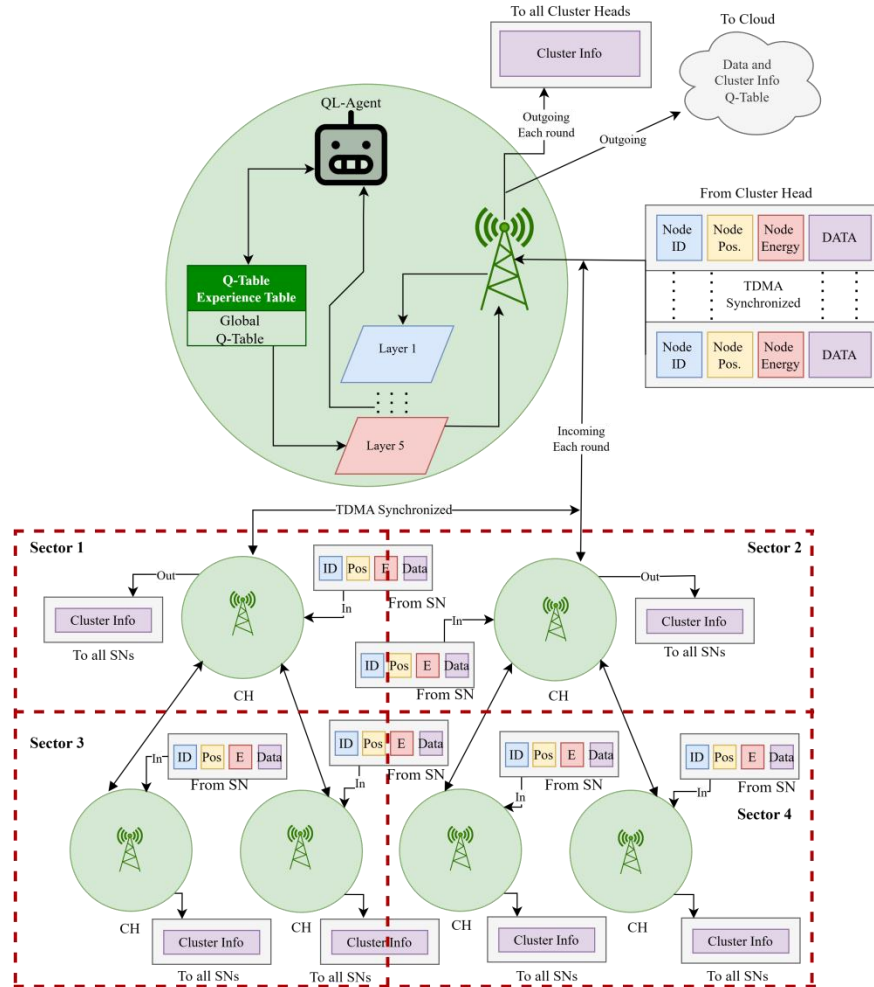
Figure 3.6.1 Centralized RLHC Deployment
