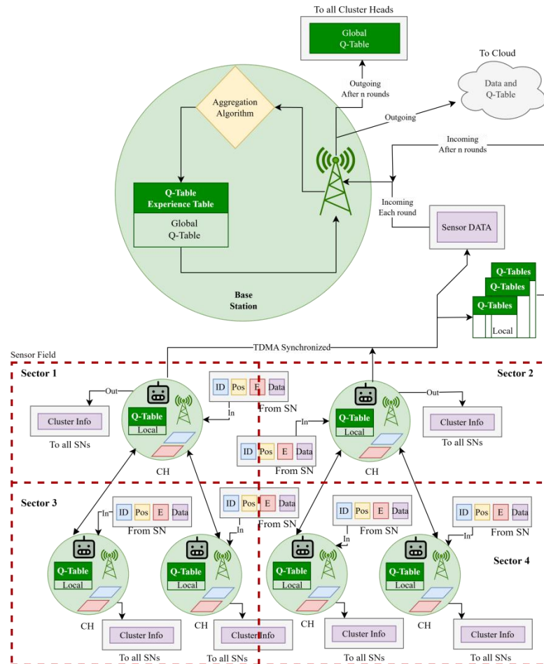
Figure 3.6.2 Federated RLHC Deployment
