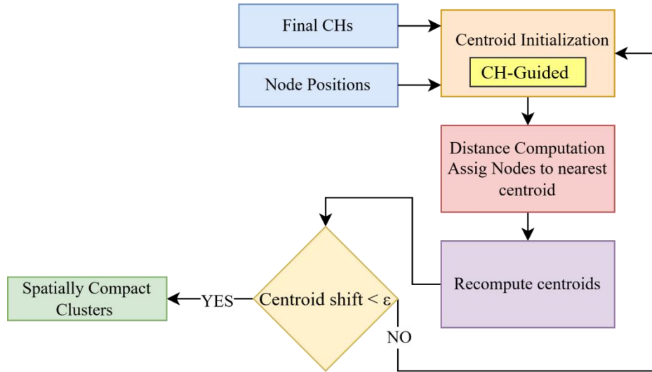
Figure 3.3.1 K-Means Algorithm
