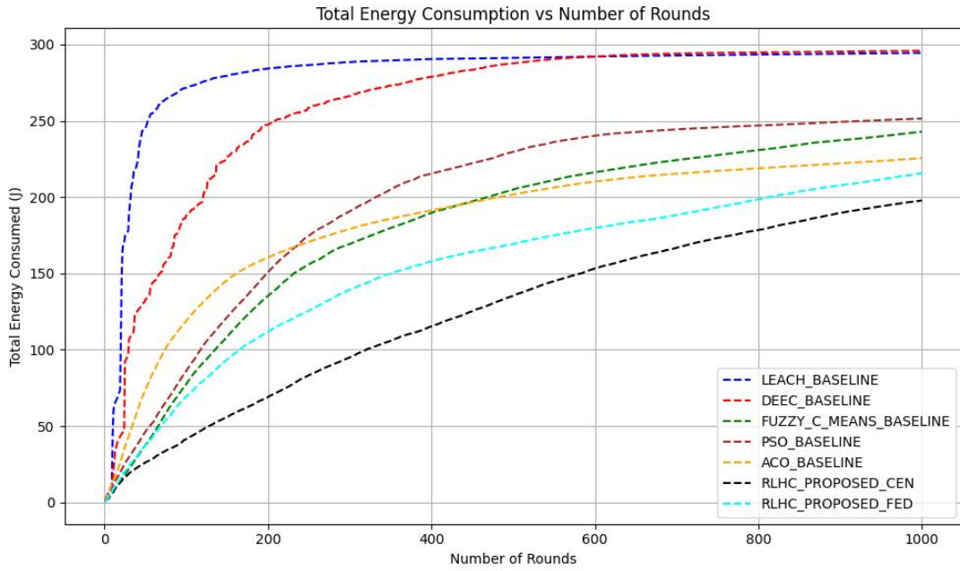
Figure 4.3.1 Total Energy Consumption
