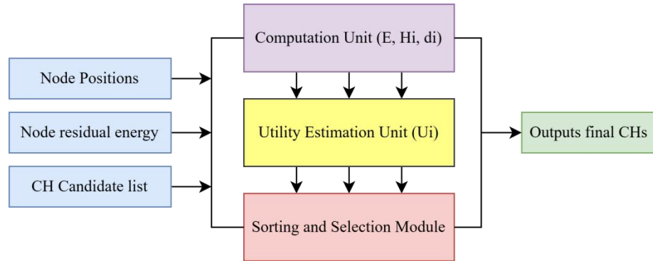
Figure 3.2.1 EEK Algorithm
