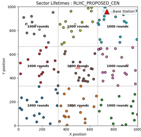
Fig 4.6 Sector-wise survival in RLHC
