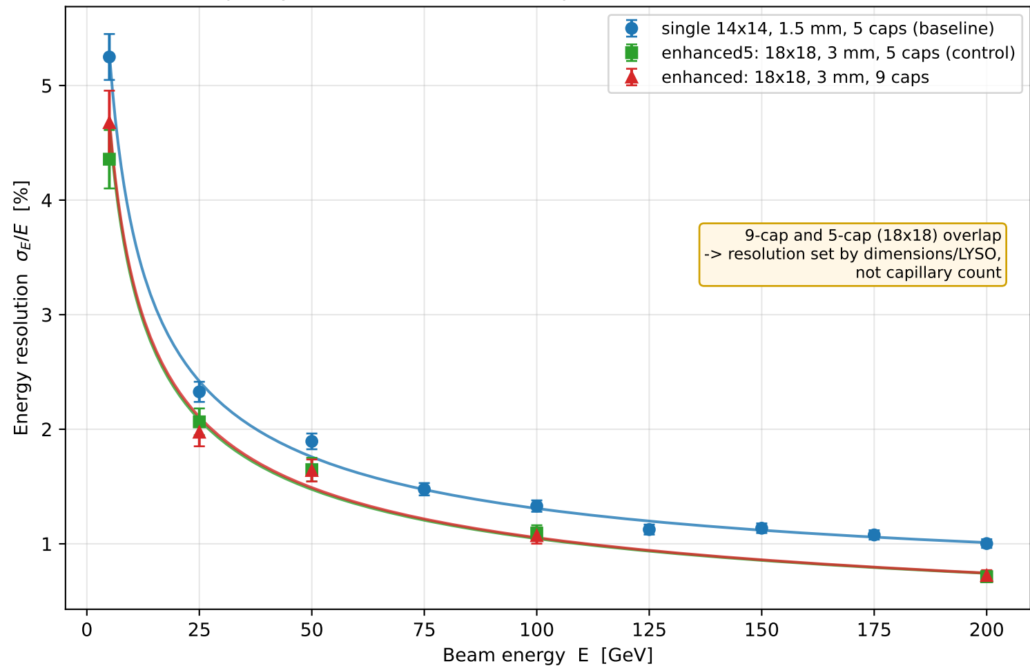
Capillary-count control: 5 vs 9 capillaries at fixed 18x18 / 3 mm
