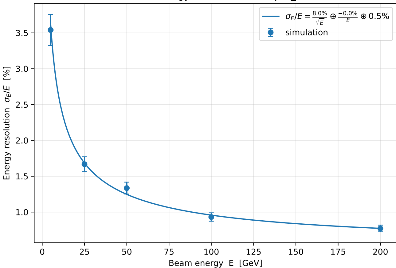
RADiCAL energy resolution (eTotLyso_MeV)
