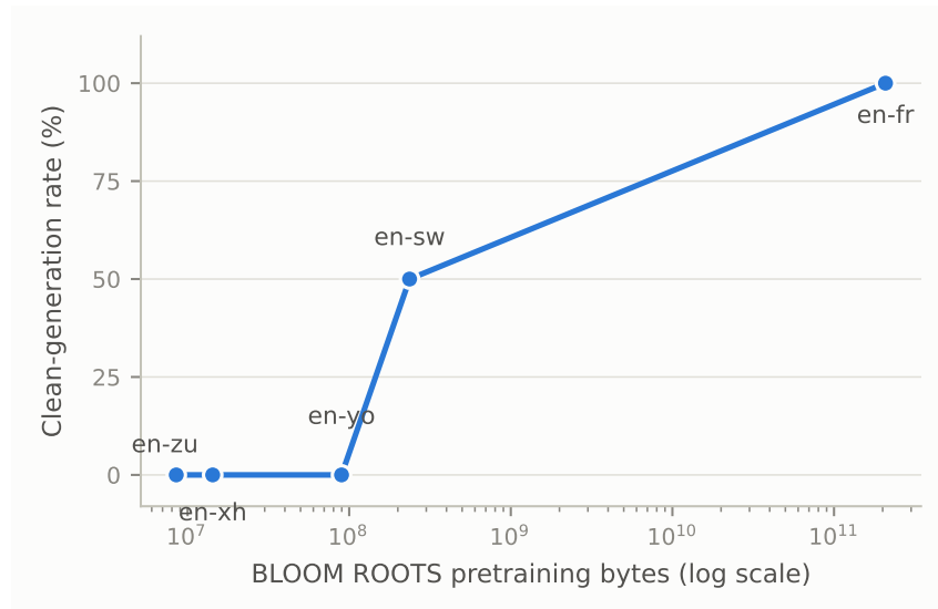
Figure 2: BLOOMZ clean-generation rate vs. ROOTS pretraining bytes (log scale), en-fr/en-sw/en-yo/en-xh/en-zu. Note the drop between en-sw and en-yo, not a smooth ramp.
