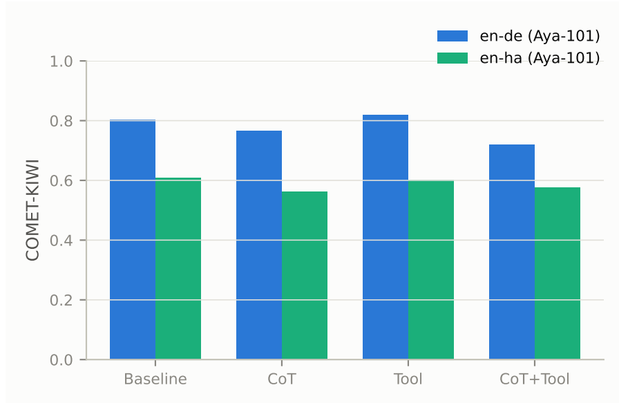
Figure 1: Phase 3 condition means (COMET-KIWI). CoT’s low score reflects the degenerate-repeat confound described above, not a clean reasoning-vs-baseline comparison.
