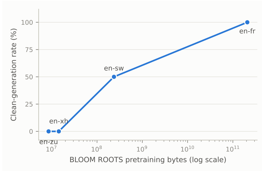
Figure 2: BLOOMZ clean-generation rate vs. ROOTS pretraining bytes (log scale), en-fr/en-sw/en-xh/en-zu.
