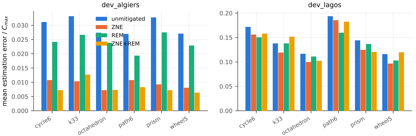
Fig. 3. Per-instance results. Pooled means conceal instance-to-instance heterogeneity, which is why inference is instance-aware. Simulator only.
