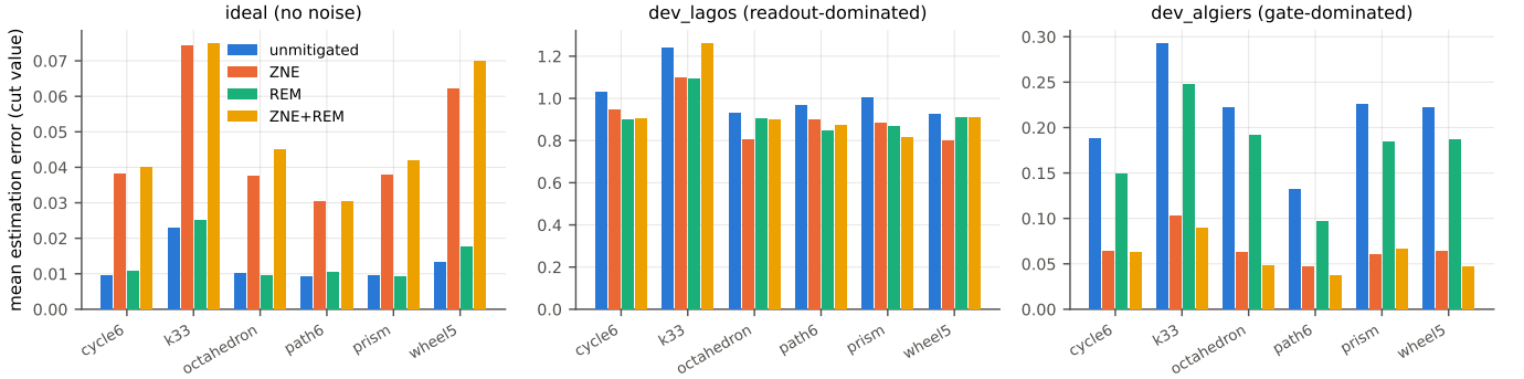
Fig. 4. Per-instance results at B = 6000 (30 seeds per bar). Pooled means conceal substantial instance-to-instance heterogeneity. Simulator only.
