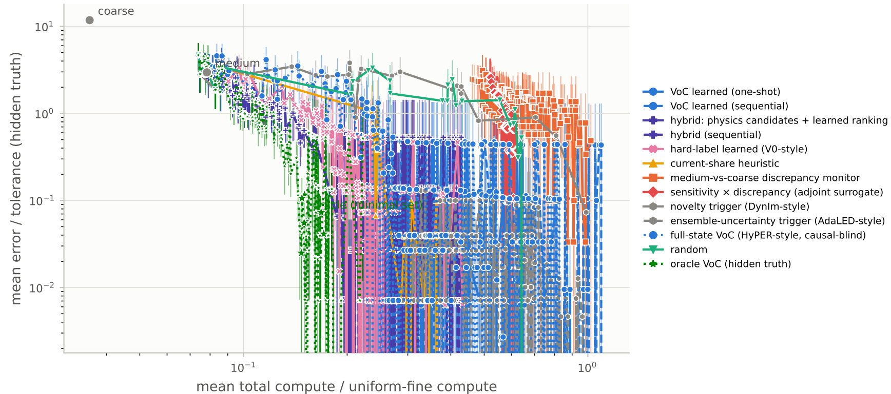
V1 main run: target spike_count (in-distribution)
