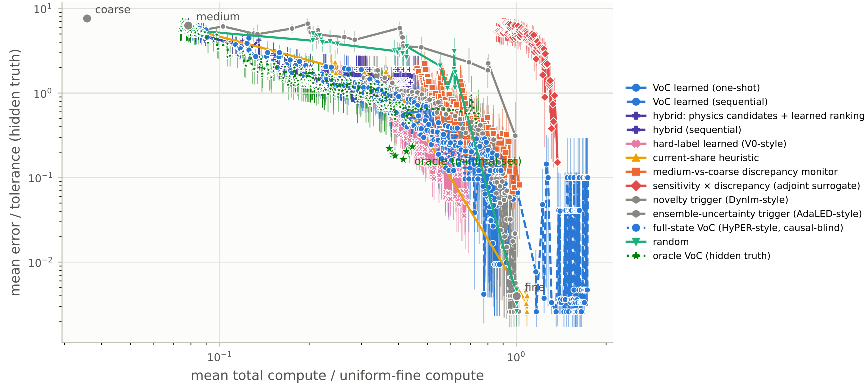
V1 main run: target v_rmse (in-distribution)
