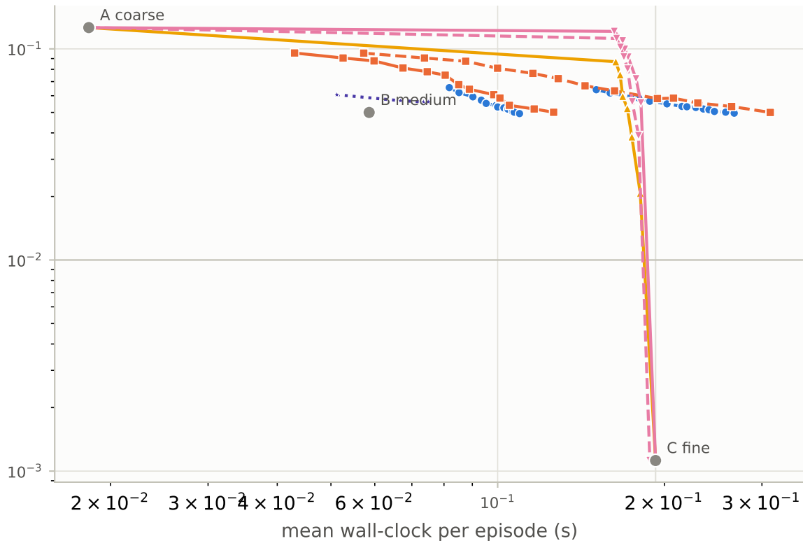
Accuracy vs wall-clock (seconds, includes controller overhead)
