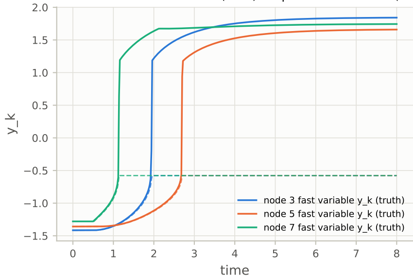
Hidden fast variables: truth (solid) vs quasi-static closure (dashed)
