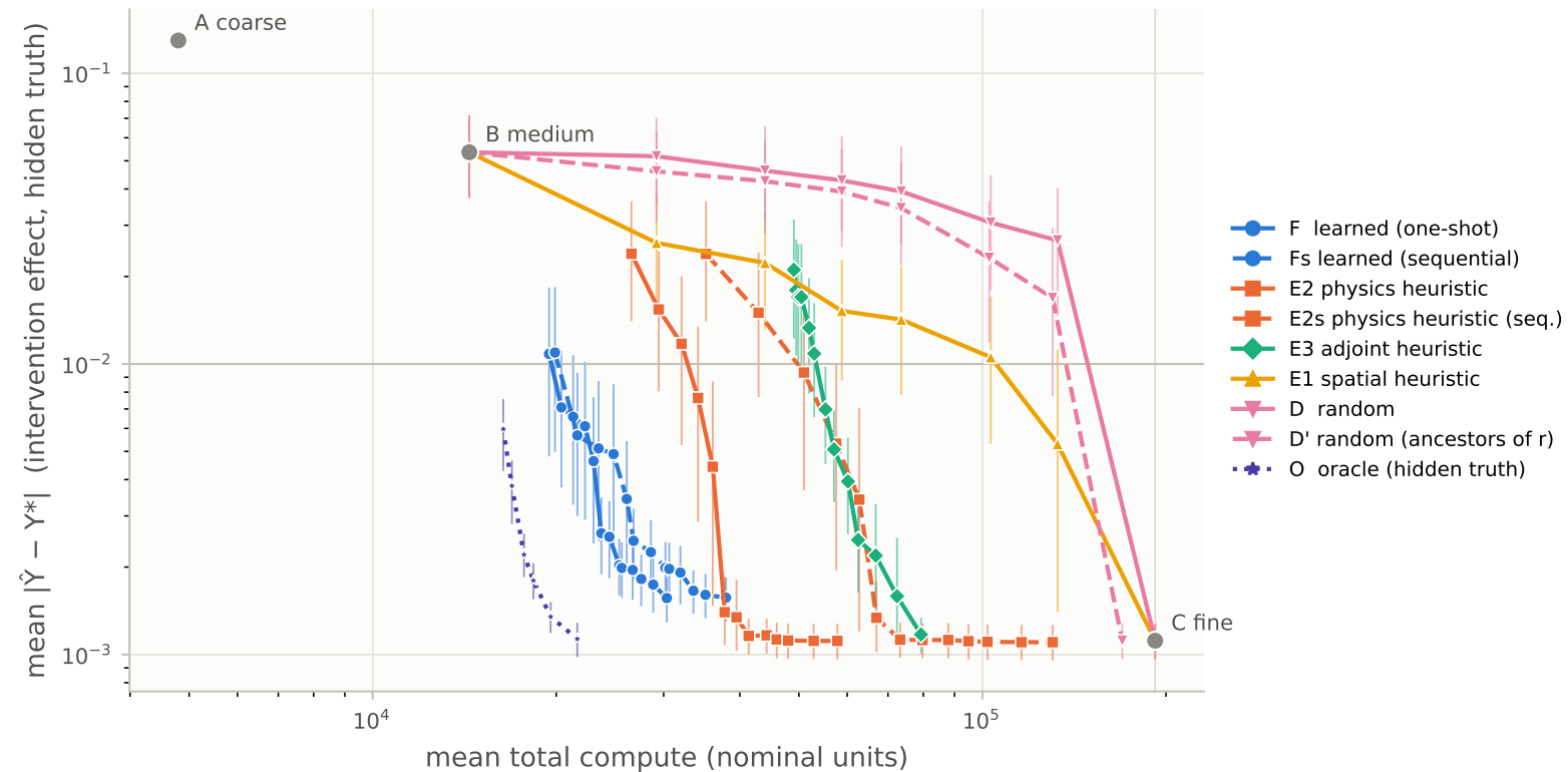
Accuracy vs compute, in-distribution test set (300 episodes, 95% bootstrap CI)
