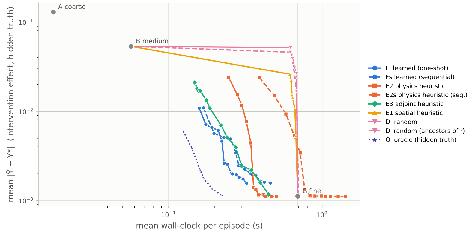
Accuracy vs wall-clock (seconds, includes controller overhead)
