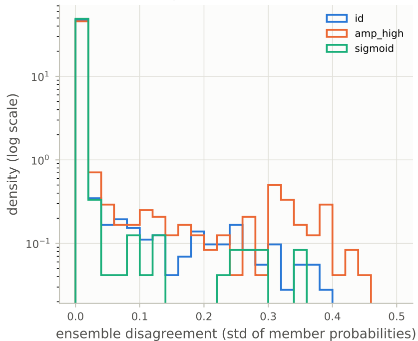
Model uncertainty in- vs out-of-distribution
