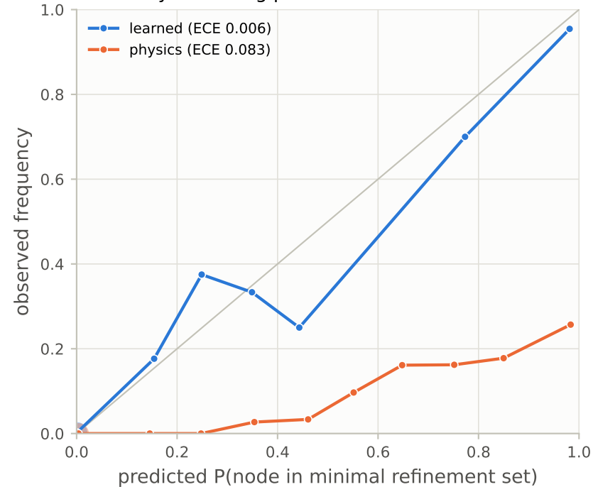
Reliability of routing probabilities
