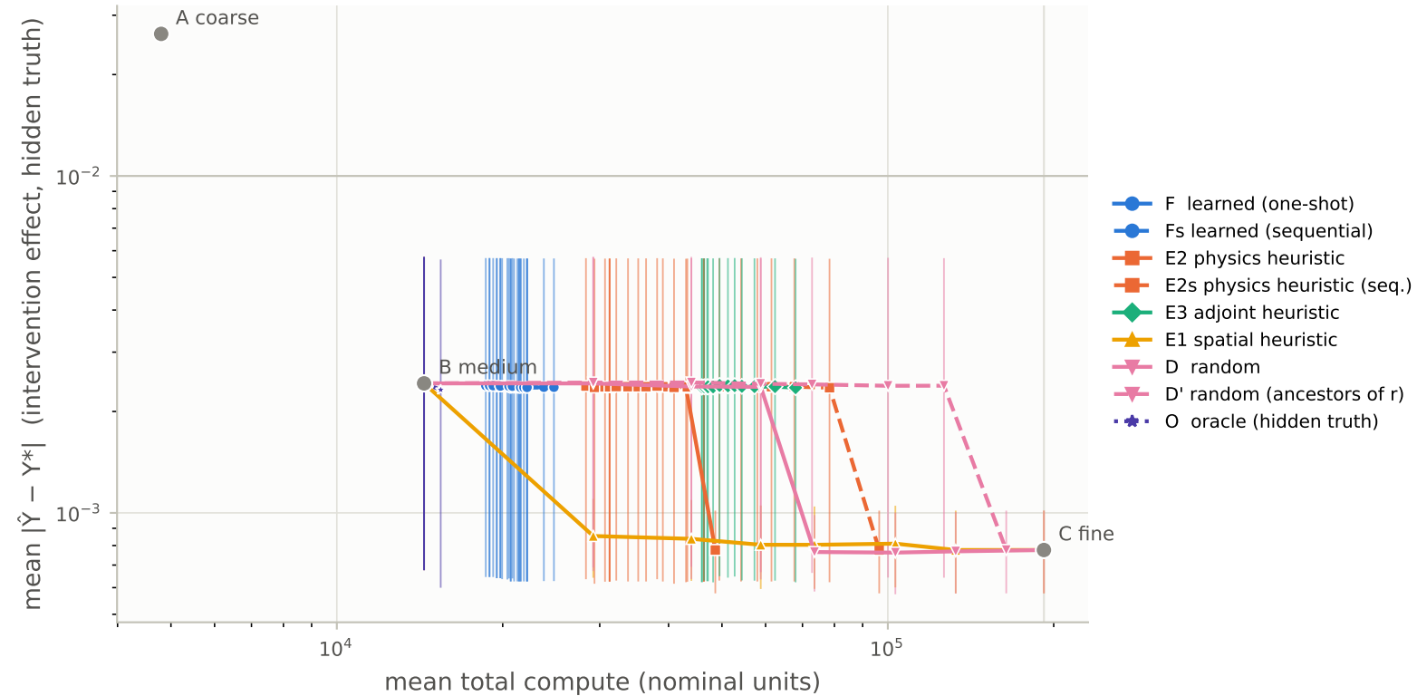
Accuracy vs compute — OOD family 'sigmoid'
