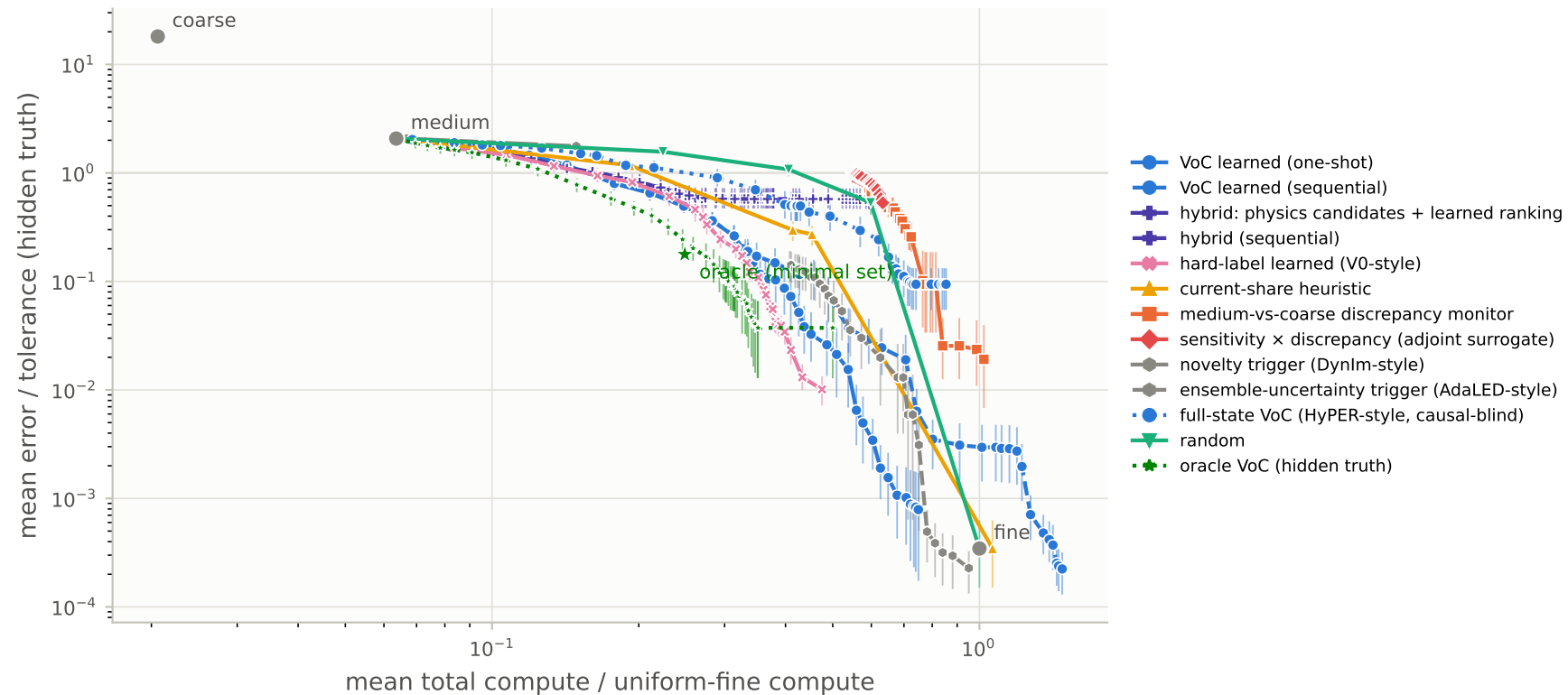
V1 main run: OOD family 'activation_rate' (pooled over targets)
