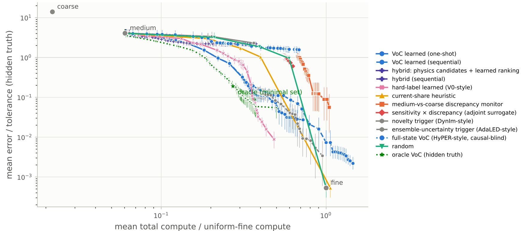
V1 main run: OOD family 'block' (pooled over targets)
