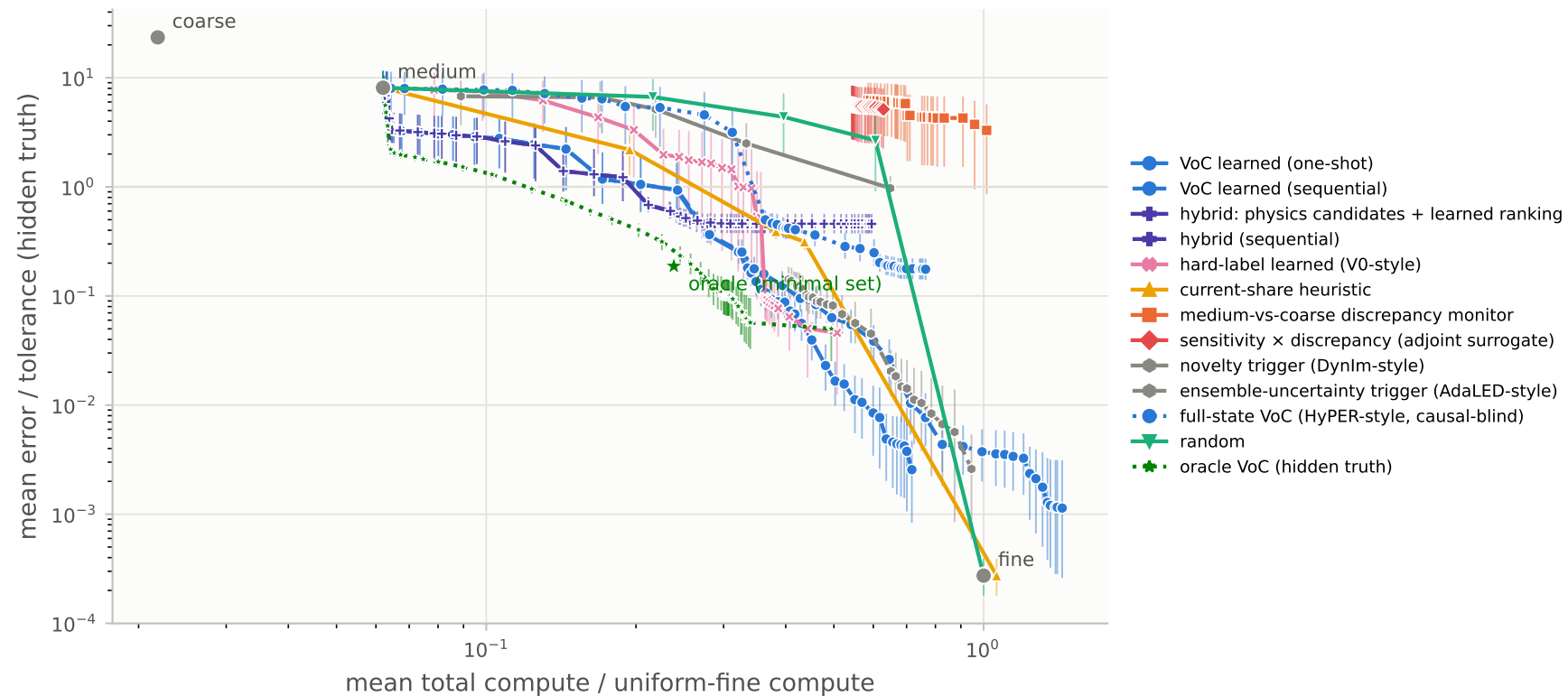
V1 main run: reserved ID set (pooled over targets)
