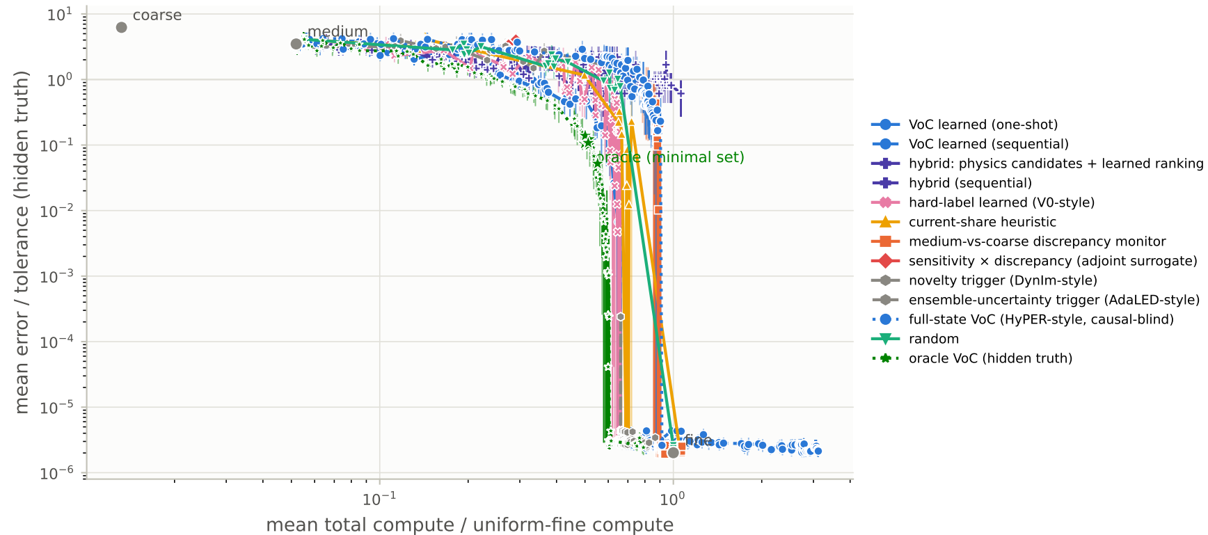
V1 main run: target recovery_fraction (in-distribution)
