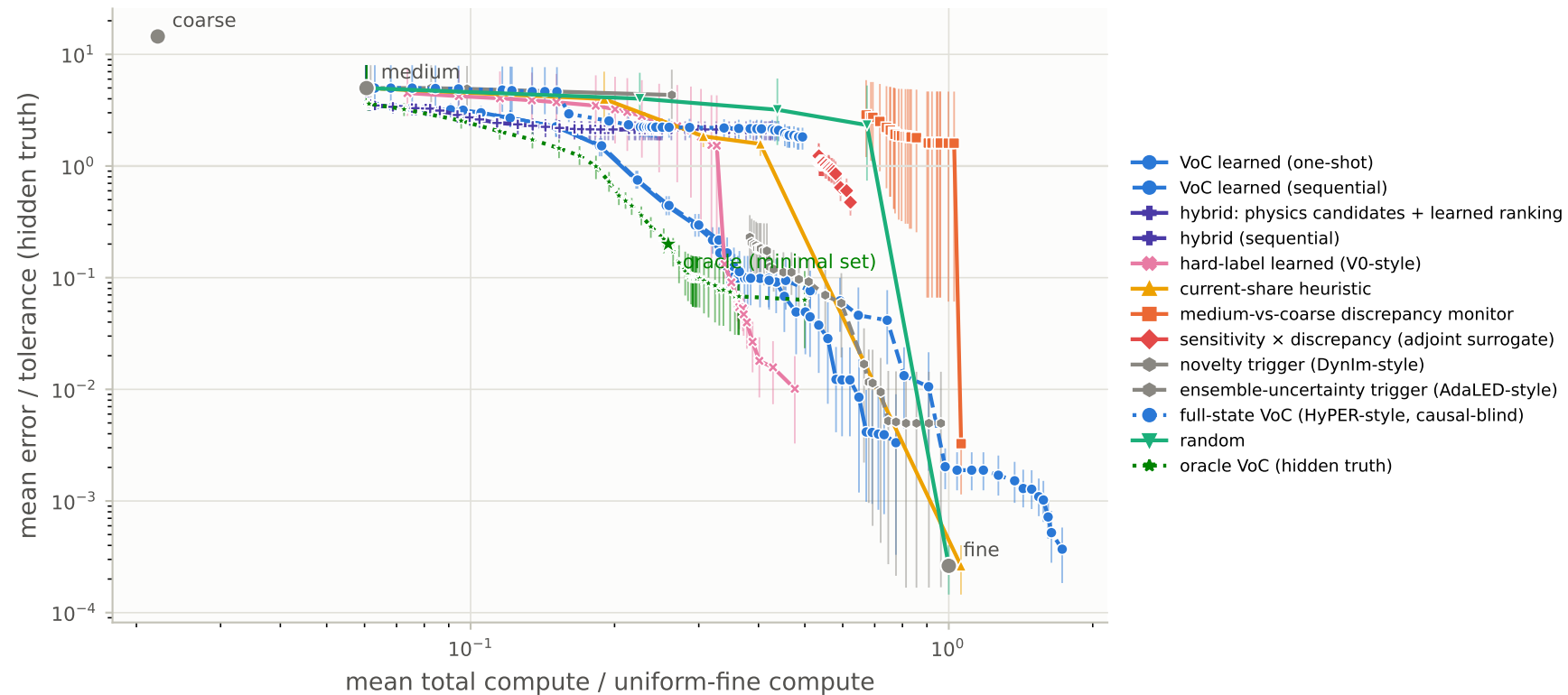
V1 pilot: OOD family 'block'
