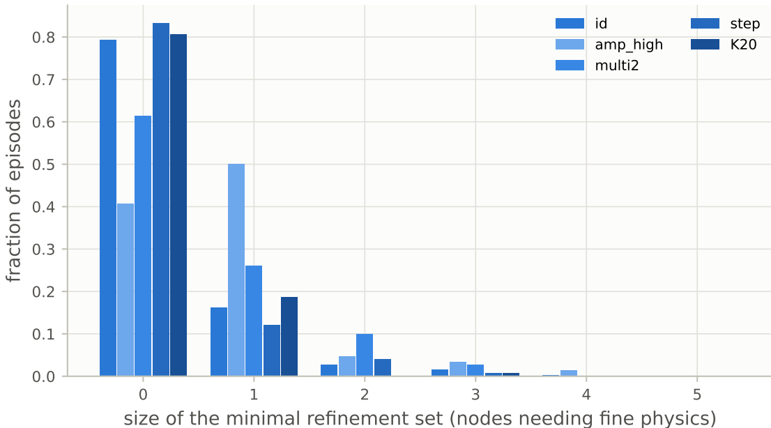
Sparsity of physical importance (H4)
