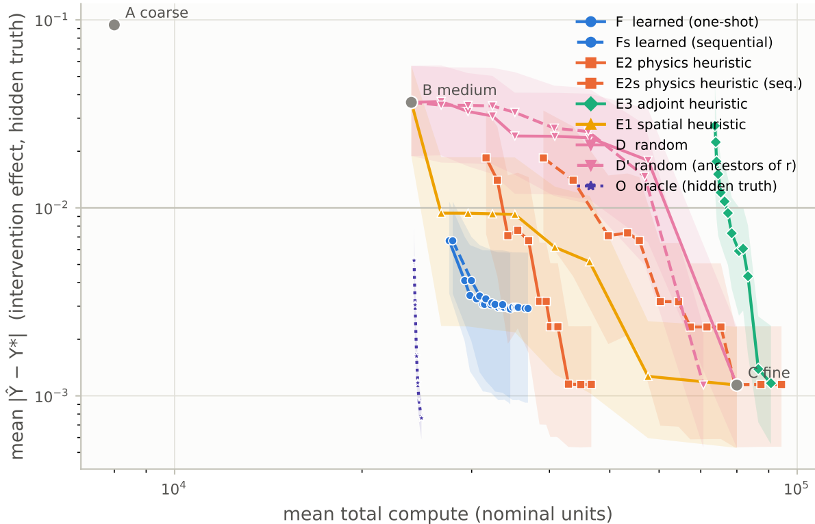
Accuracy vs compute — OOD family 'K20'
