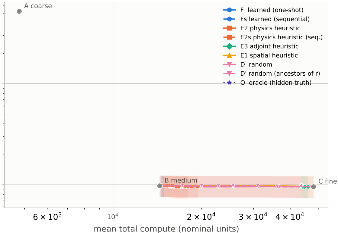
Accuracy vs compute — OOD family 'negative'
