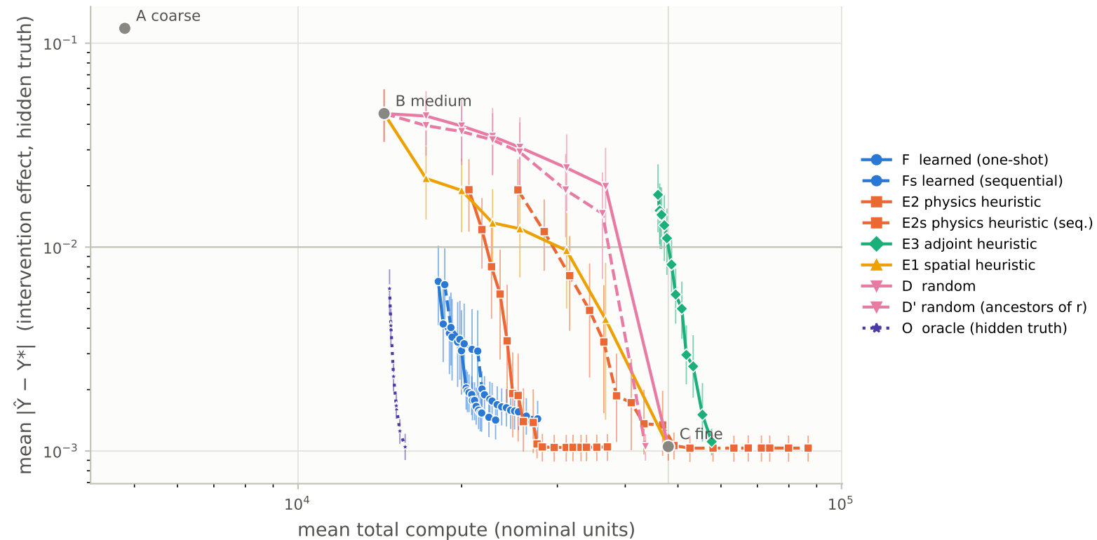
Accuracy vs compute, in-distribution test set (400 episodes, 95% bootstrap CI)
