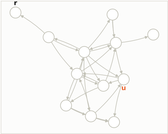
learned (seq.): |err| 0.009, cost 14400
