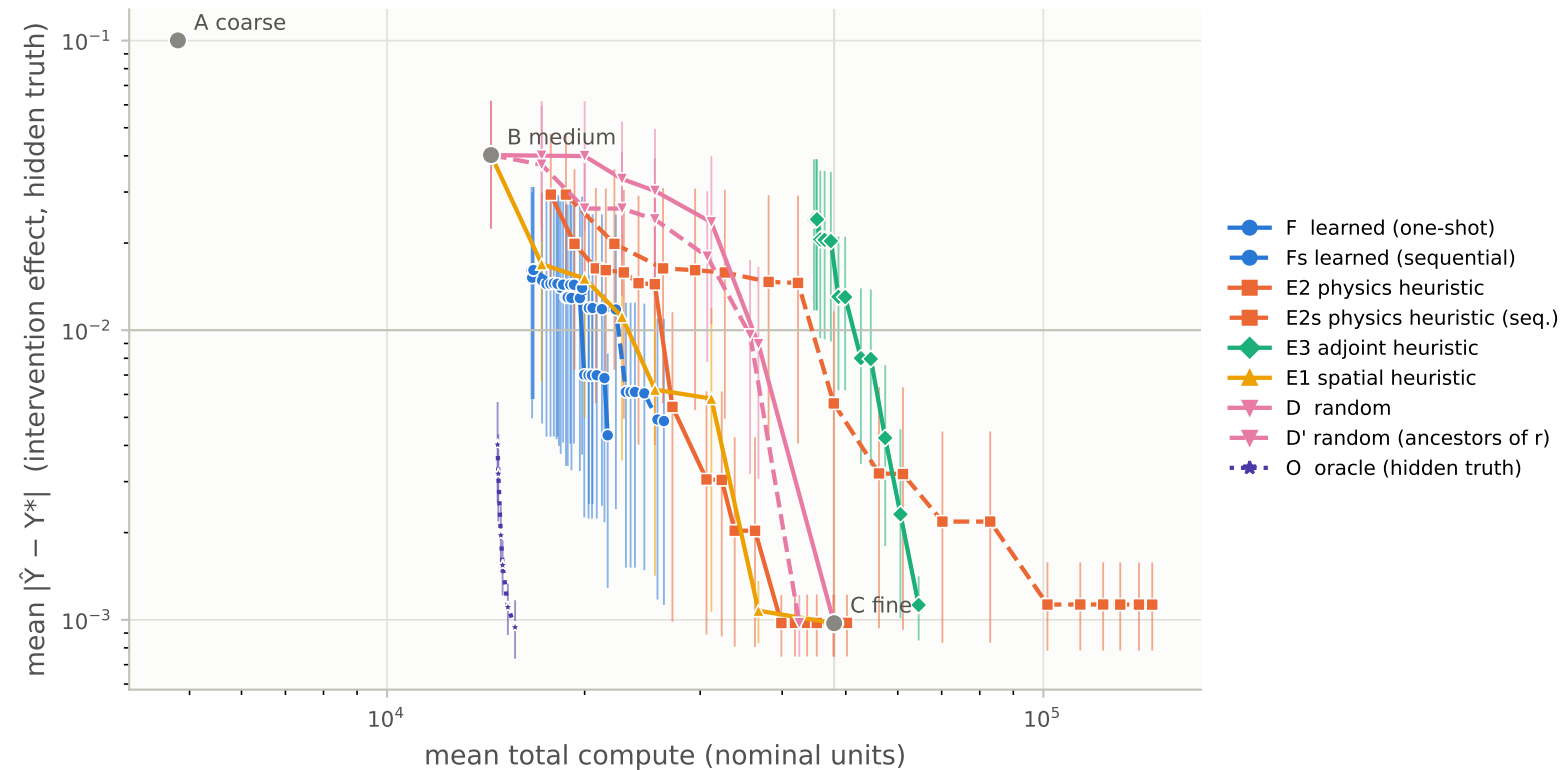
Accuracy vs compute — OOD family 'sigma06'
