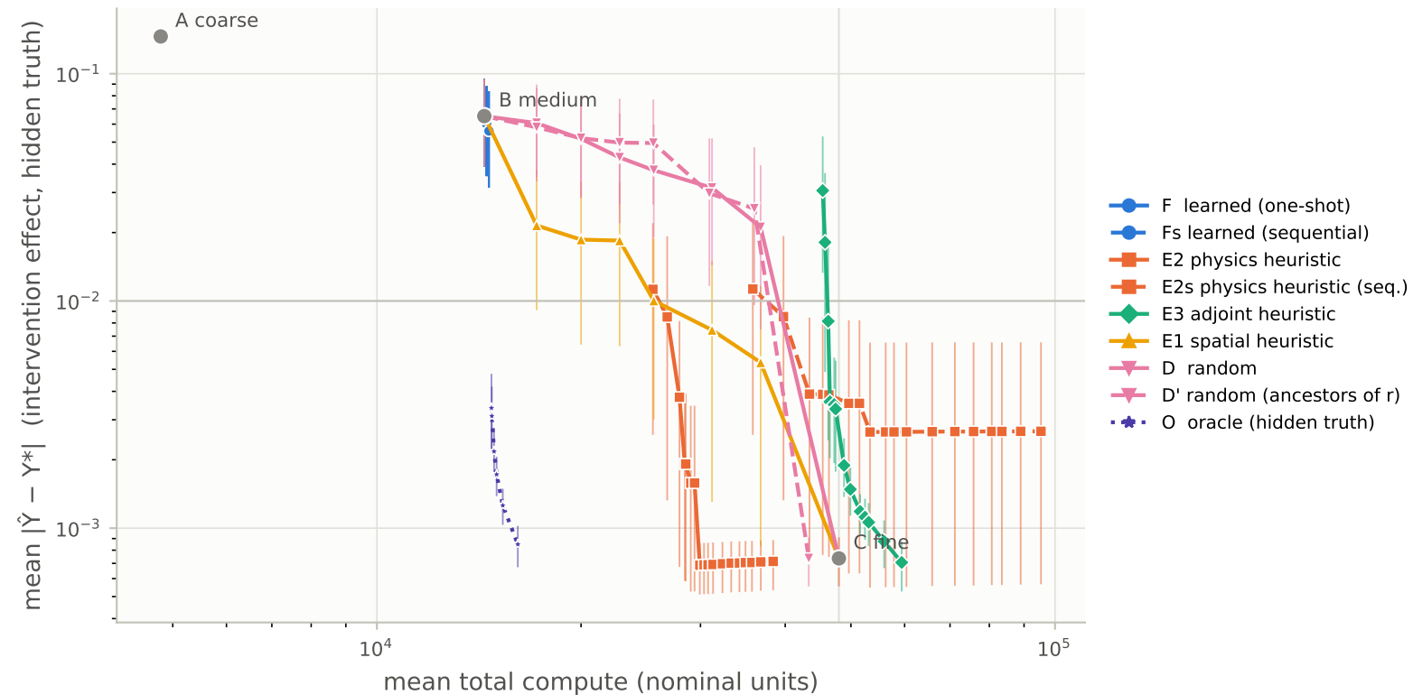
Accuracy vs compute — OOD family 'step'
