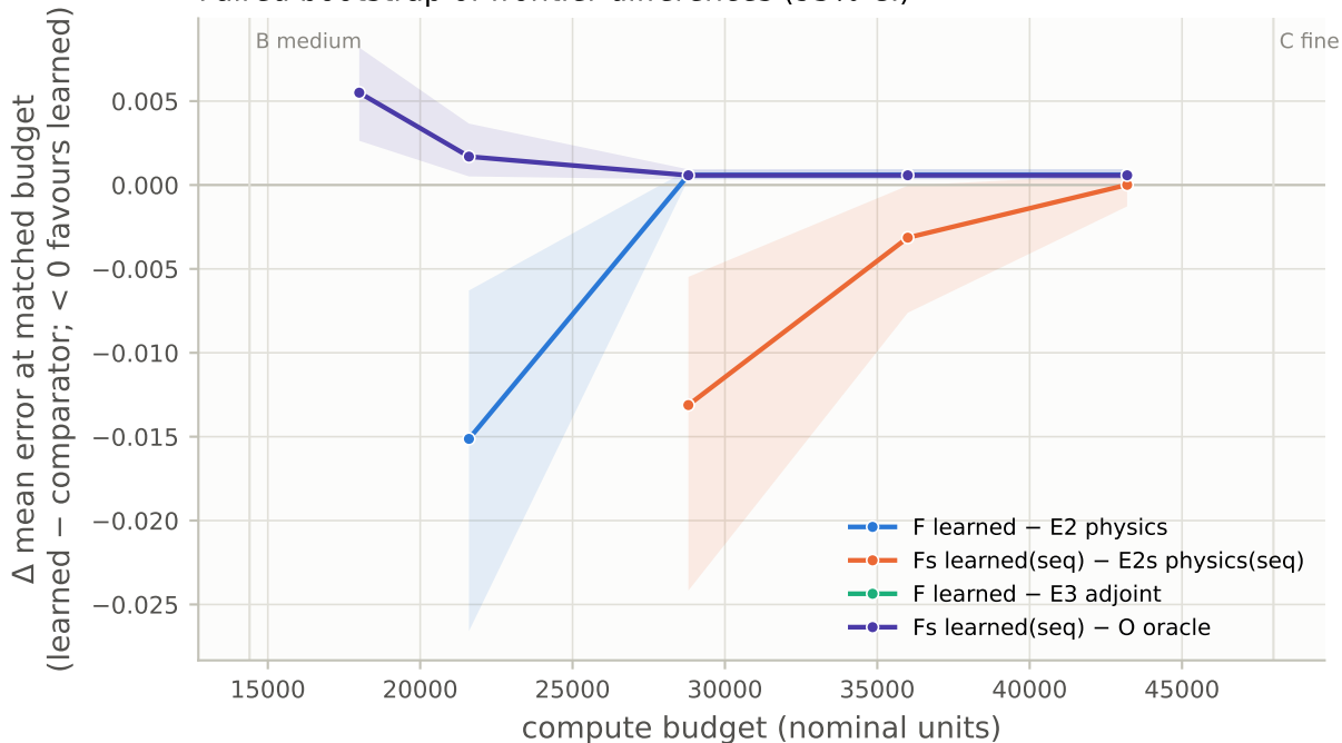
Paired bootstrap of frontier differences (95% CI)
