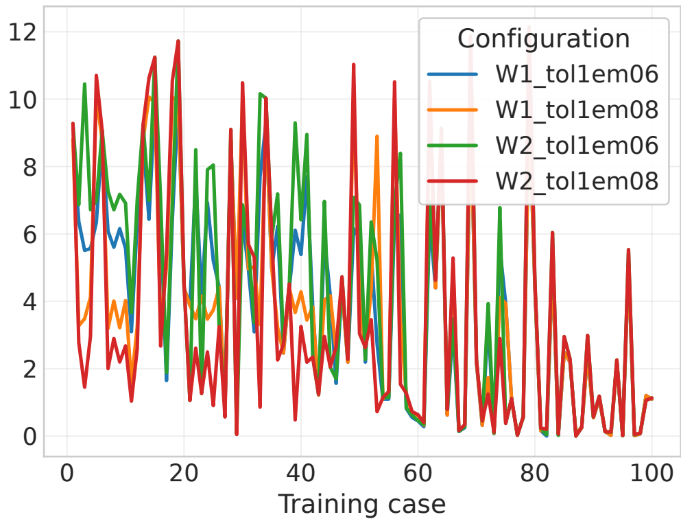
Training loss
