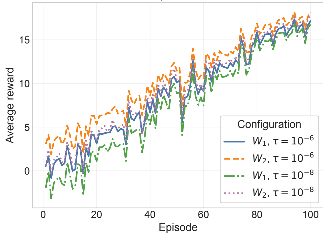
Dense systems: reward
