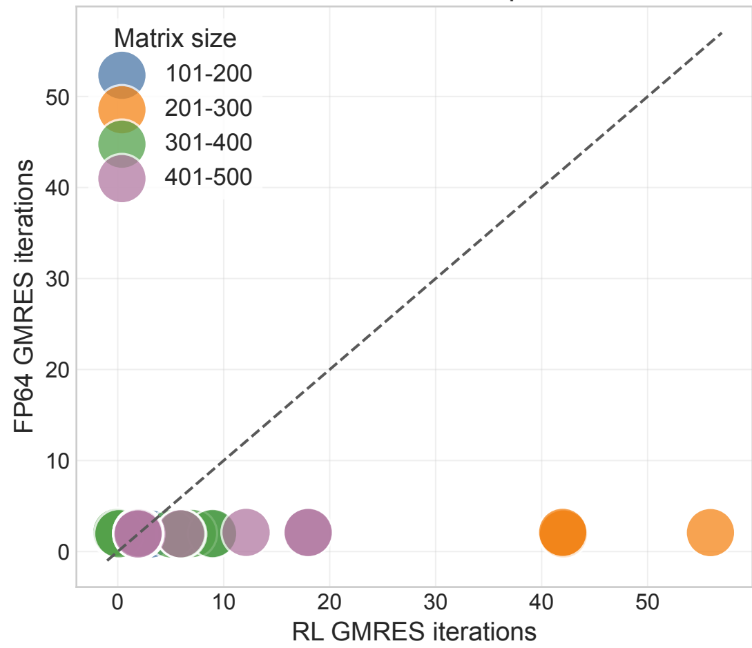
GMRES iteration comparison
