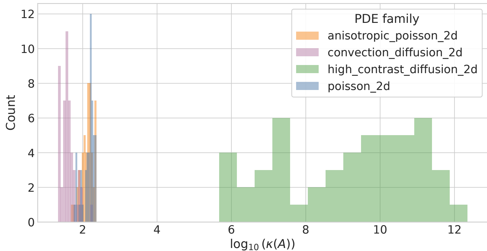
PDE dataset condition-number distribution
